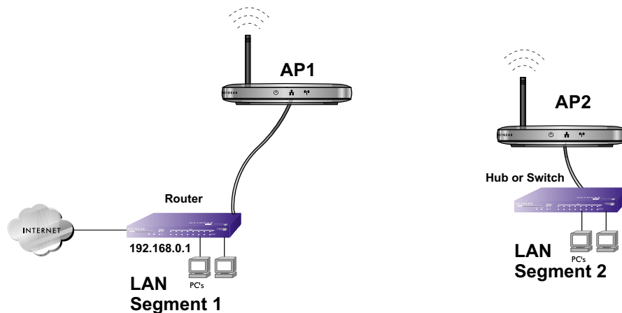
Figure 5-3: Wireless Bridging
