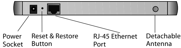
Figure 2-2: WG602 v2 rear panel
