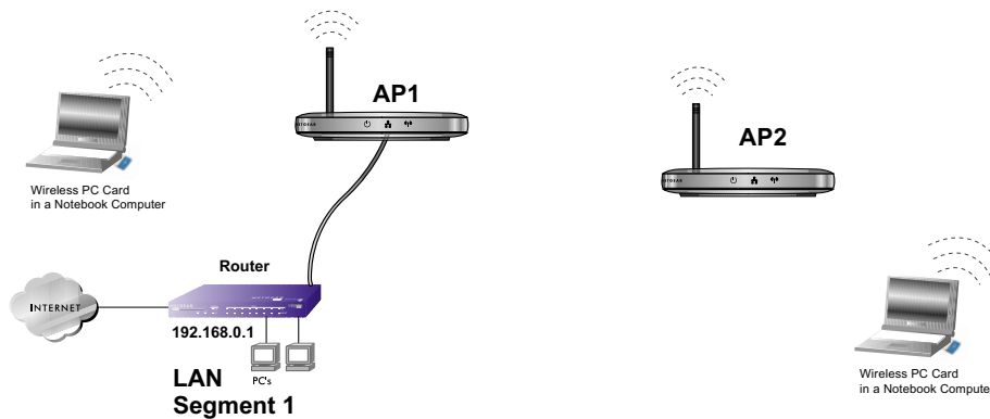
Figure 5-2: Wireless Repeater
