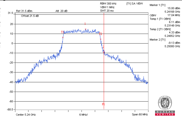
802.11ac(VHT20)_Chain0 / CH48
