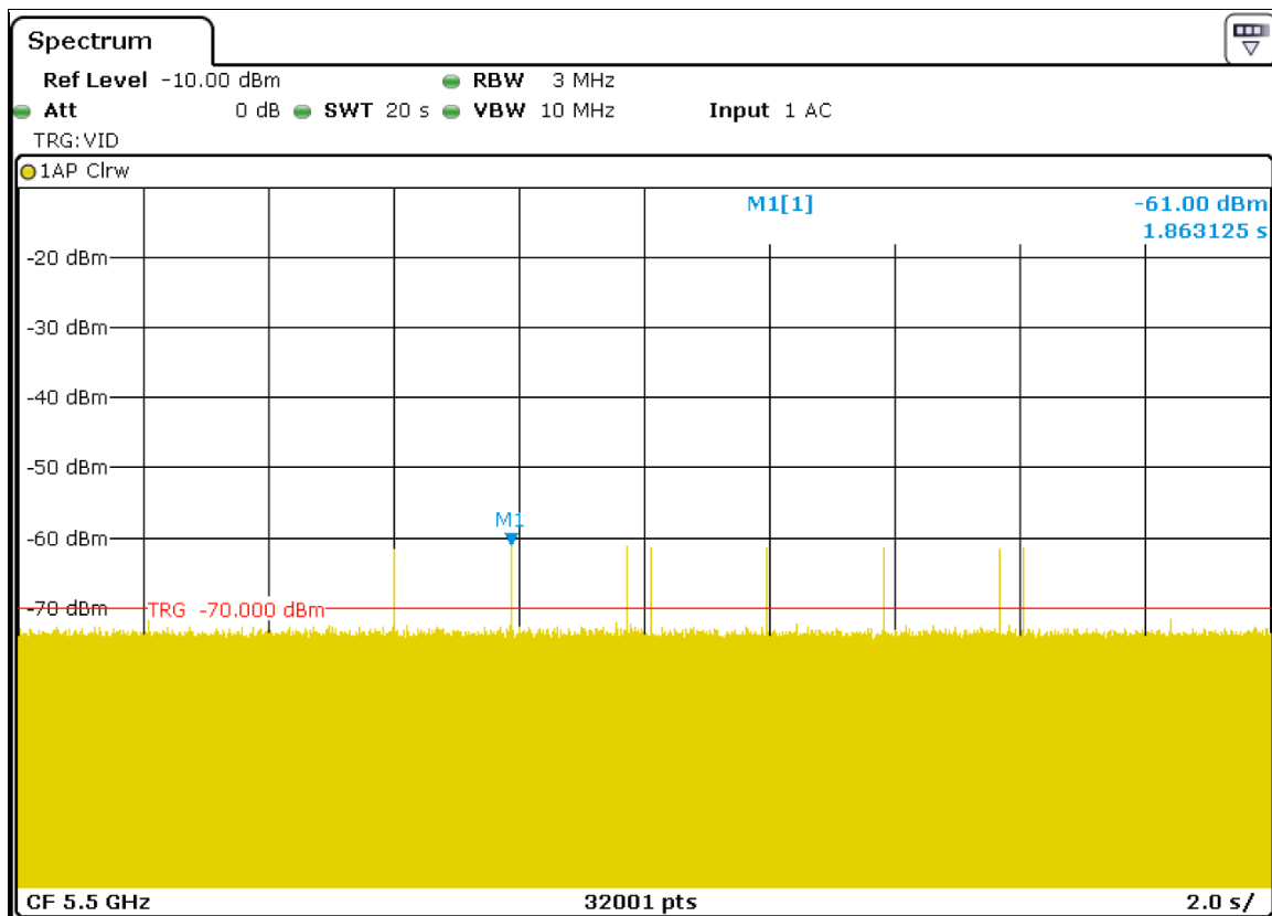
Radar Signal 5
