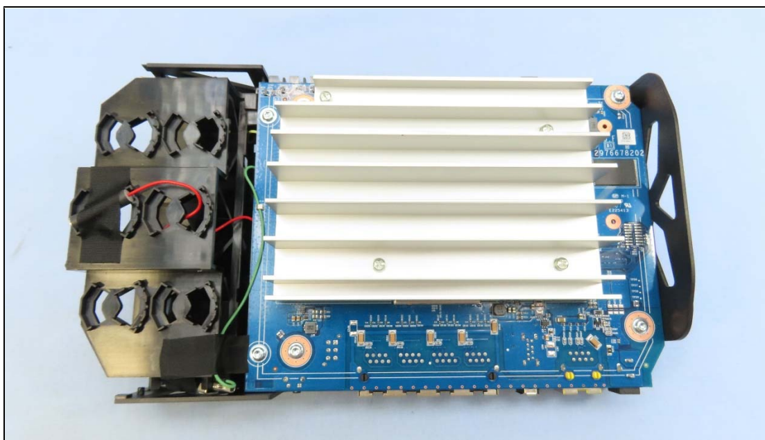
Antenna Option 2
