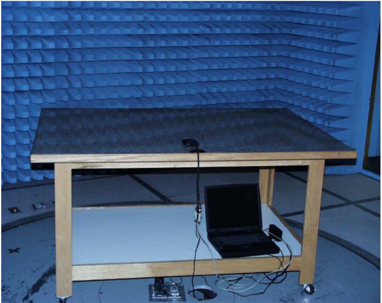
Front view of the test setup
