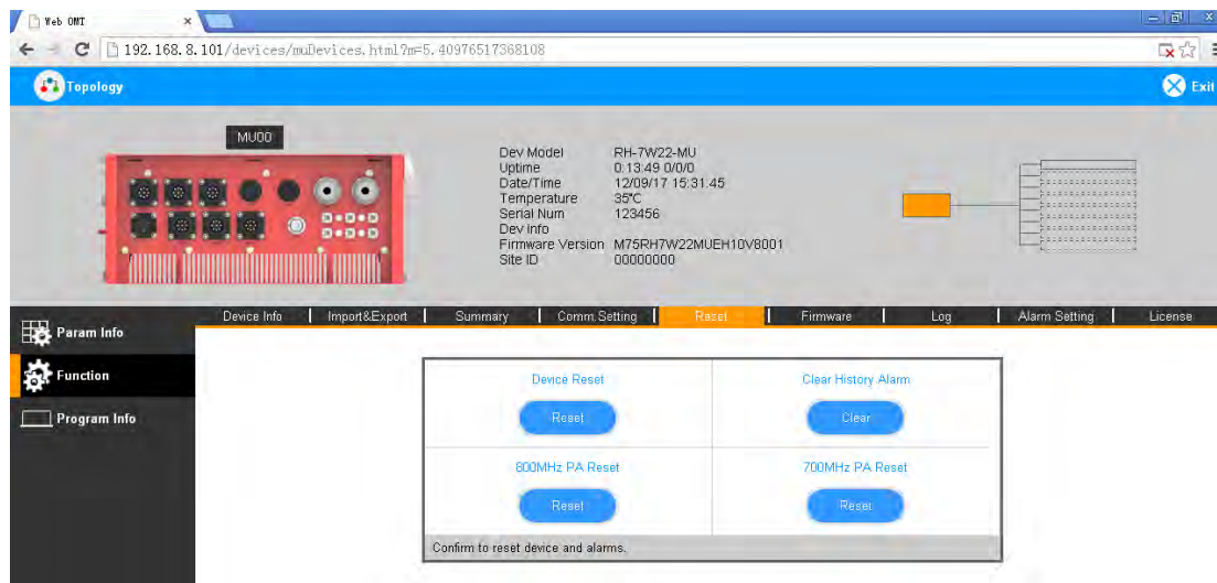
Figure 34: Function –Reset
