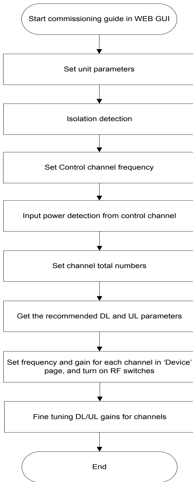
Figure 13: Commissioning Procedure
