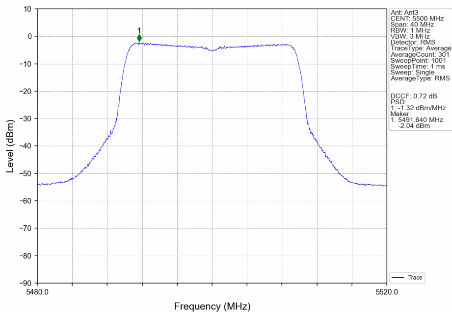
802.11ax(HEW20)_LCH_5500MHz_RU26_Mid_Ant3_NTNV
