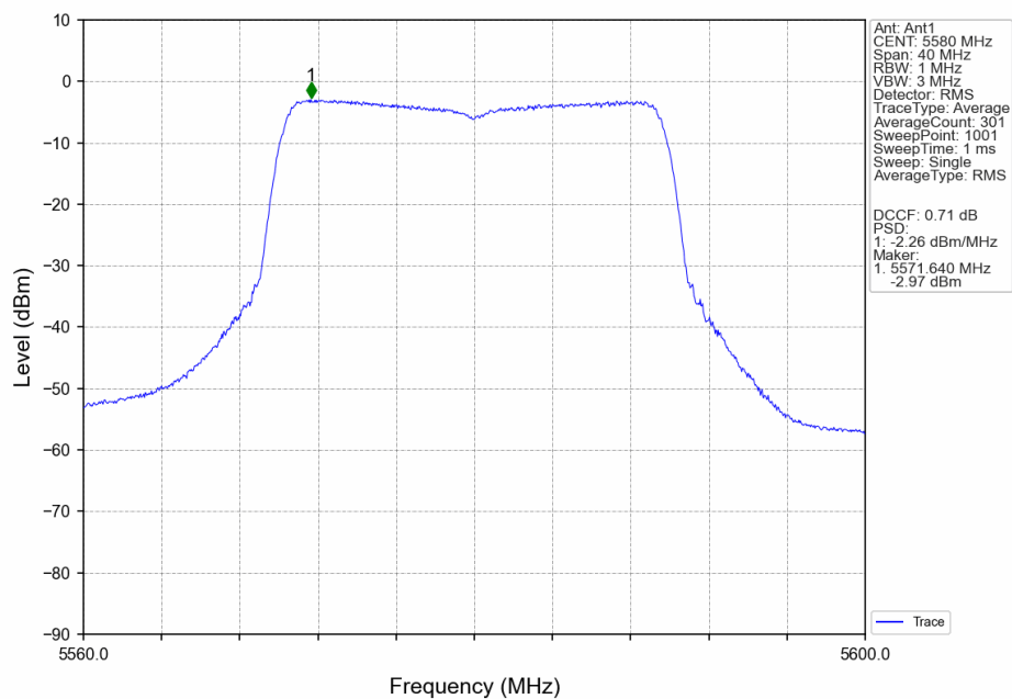
802.11ax(HEW20)_MCH_5580MHz_RU242_Left_Ant1_NTNV
