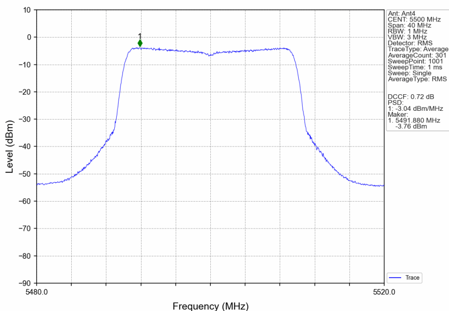
802.11ax(HEW20)_LCH_5500MHz_RU26_Right_Ant4_NTNV
