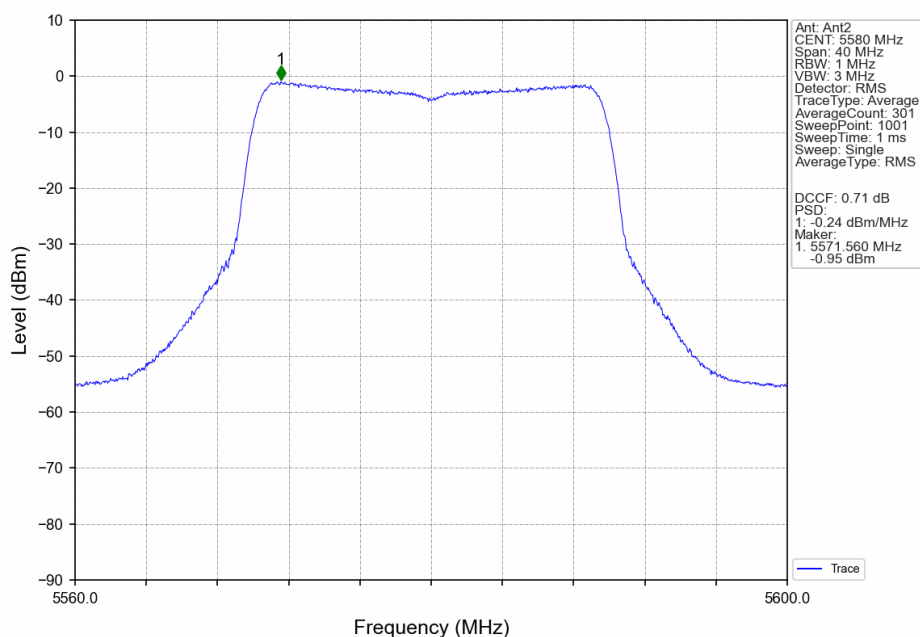
802.11ax(HEW20)_MCH_5580MHz_RU26_Right_Ant2_NTNV
