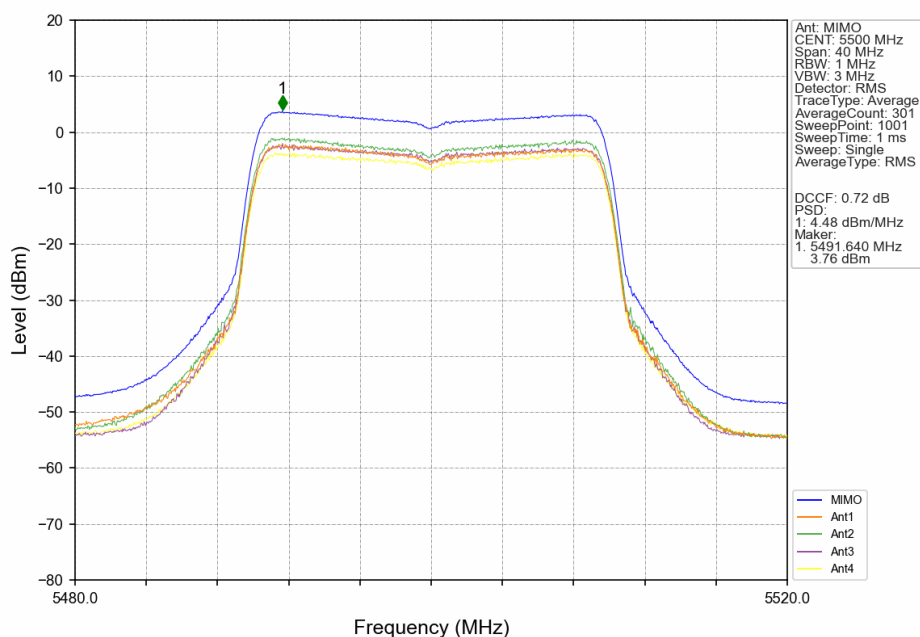
802.11ax(HEW20)_LCH_5500MHz_RU26_Mid_MIMO_NTNV
