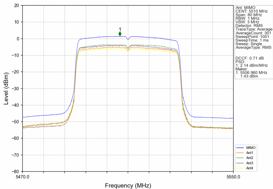
802.11ax(HEW40)_LCH_5510MHz_RU484_Left_MIMO_NTNV
