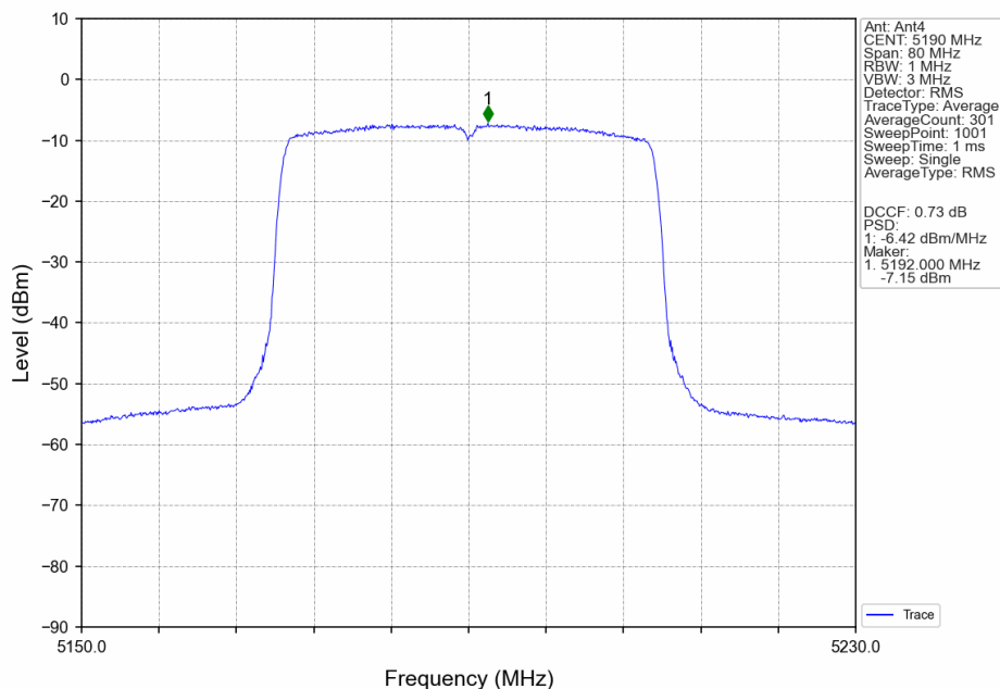
802.11ax(HEW40)_LCH_5190MHz_RU26_Mid_MIMO_NTNV
