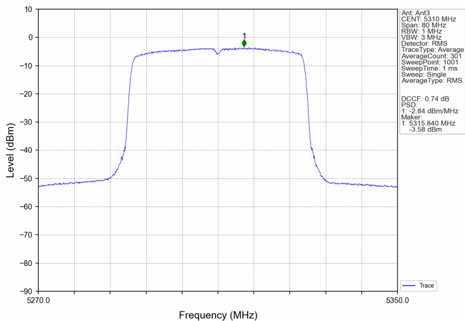
802.11ax(HEW40)_HCH_5310MHz_RU26_Mid_Ant3_NTNV
