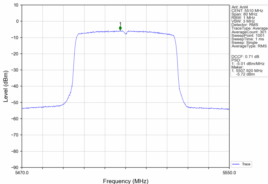
802.11ax(HEW40)_LCH_5510MHz_RU26_Mid_MIMO_NTNV
