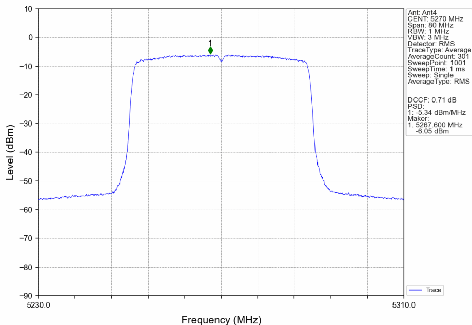
802.11ax(HEW40)_LCH_5270MHz_RU26_Mid_MIMO_NTNV
