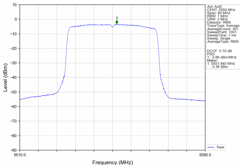
802.11ax(HEW40)_MCH_5550MHz_RU26_Left_Ant2_NTNV
