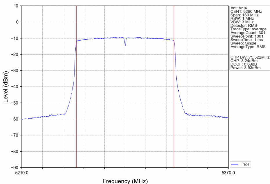
802.11ac(VHT80)_MCH_5290MHz_Ant4_NTNV
