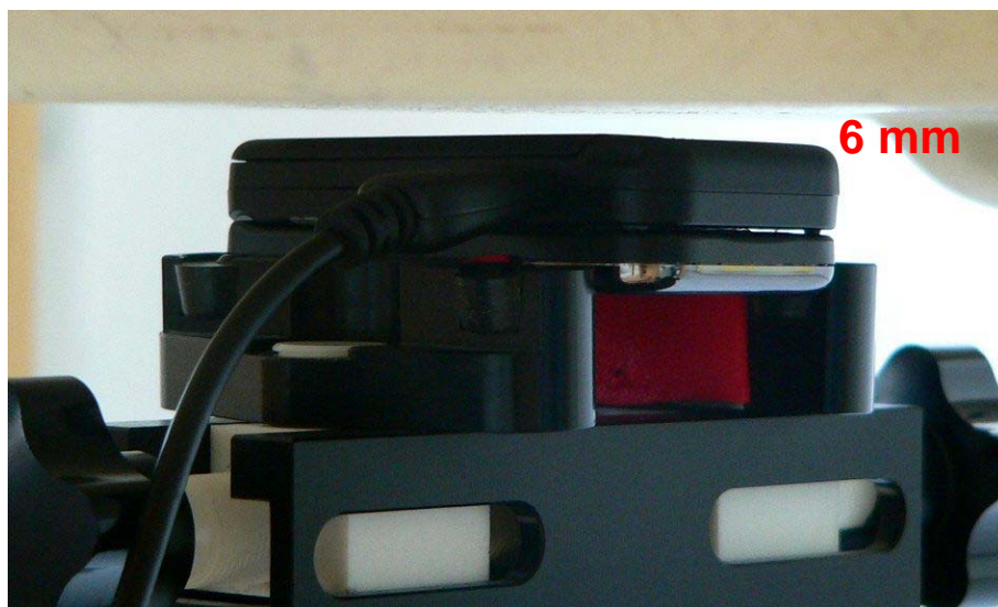
Fig. 25: Body worn configuration, GPRS (Class 8) with data cable, antenna towards the phantom.
