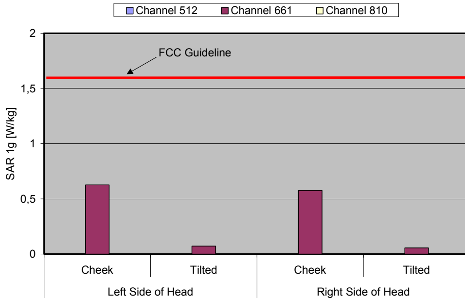
Fig. 8: The measured head phantom SAR values for the BenQ AF51 for PCS 1900 in comparison to the FCC exposure limit.
