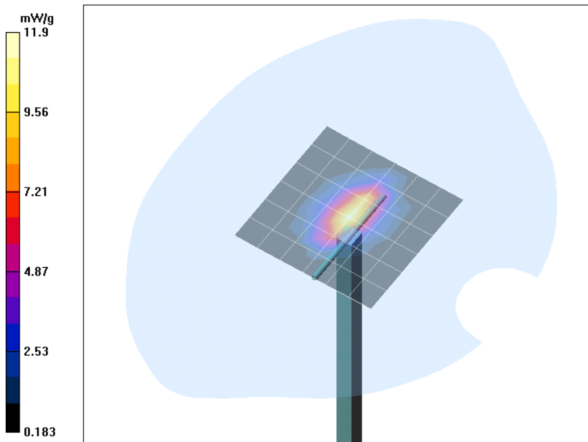
Fig. 11: Validation measurement 1900 MHz body (December 07, 2005), coarse grid. Ambient Temperature: 22.0° C, Liquid Temperature: 21.2° C.
