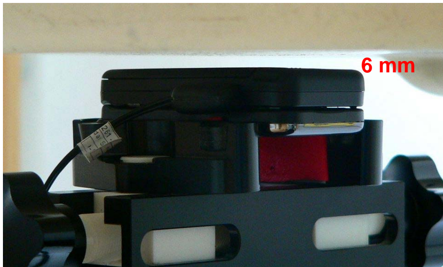
Fig. 24: Body worn configuration, GSM with headset, antenna towards the phantom.
