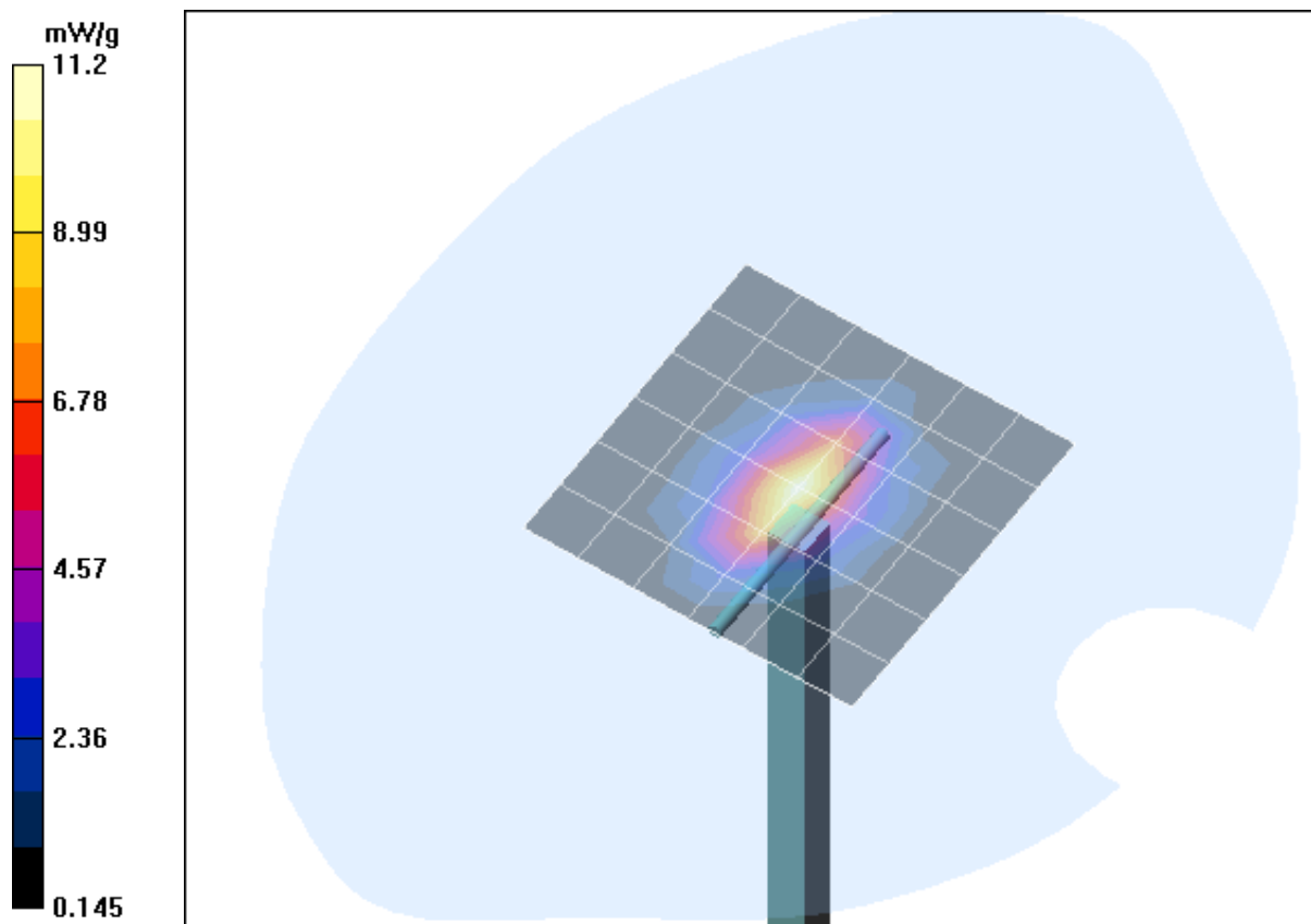
Fig. 10: Validation measurement 1900 MHz Head (December 05, 2005), coarse grid. Ambient Temperature: 21.7° C, Liquid Temperature: 21.2° C.
