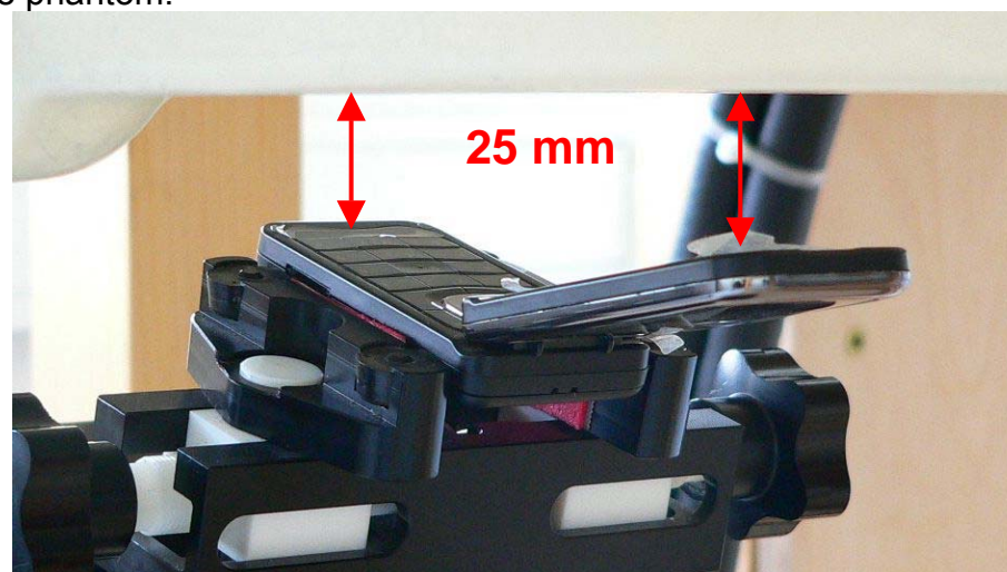
Fig. 26: Body worn configuration, PTT mode (Class 8), display towards the phantom.
