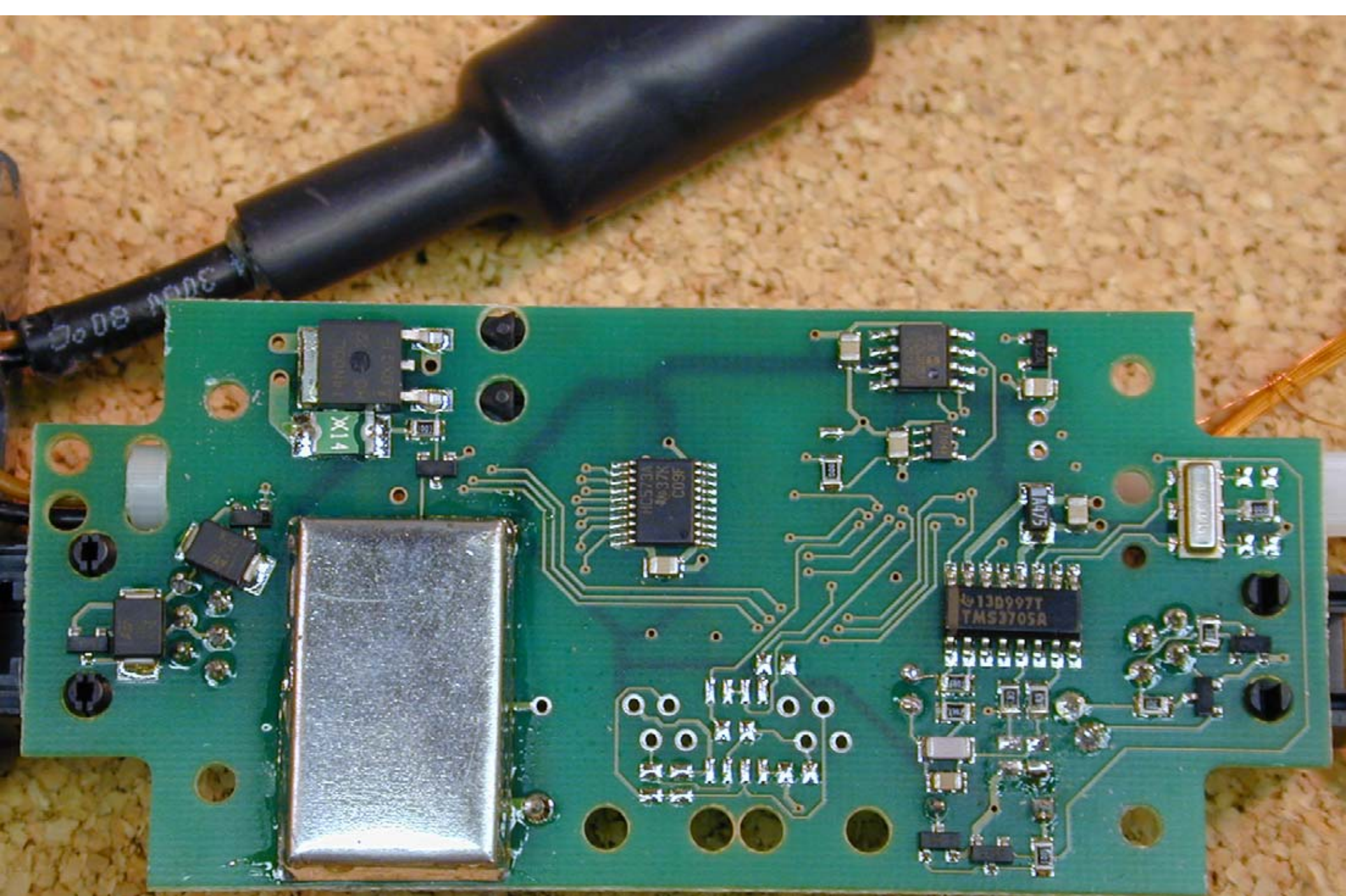
PCB bottom - Int. Antenna
