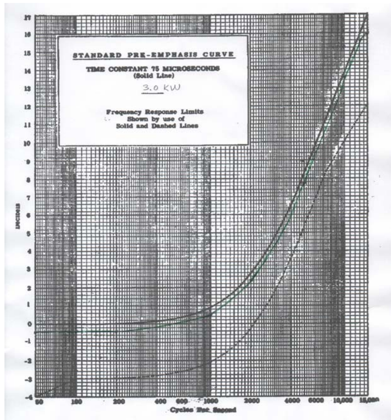
AURAL FREQUENCY RESPONSE GRAPH WITH LIMITS
