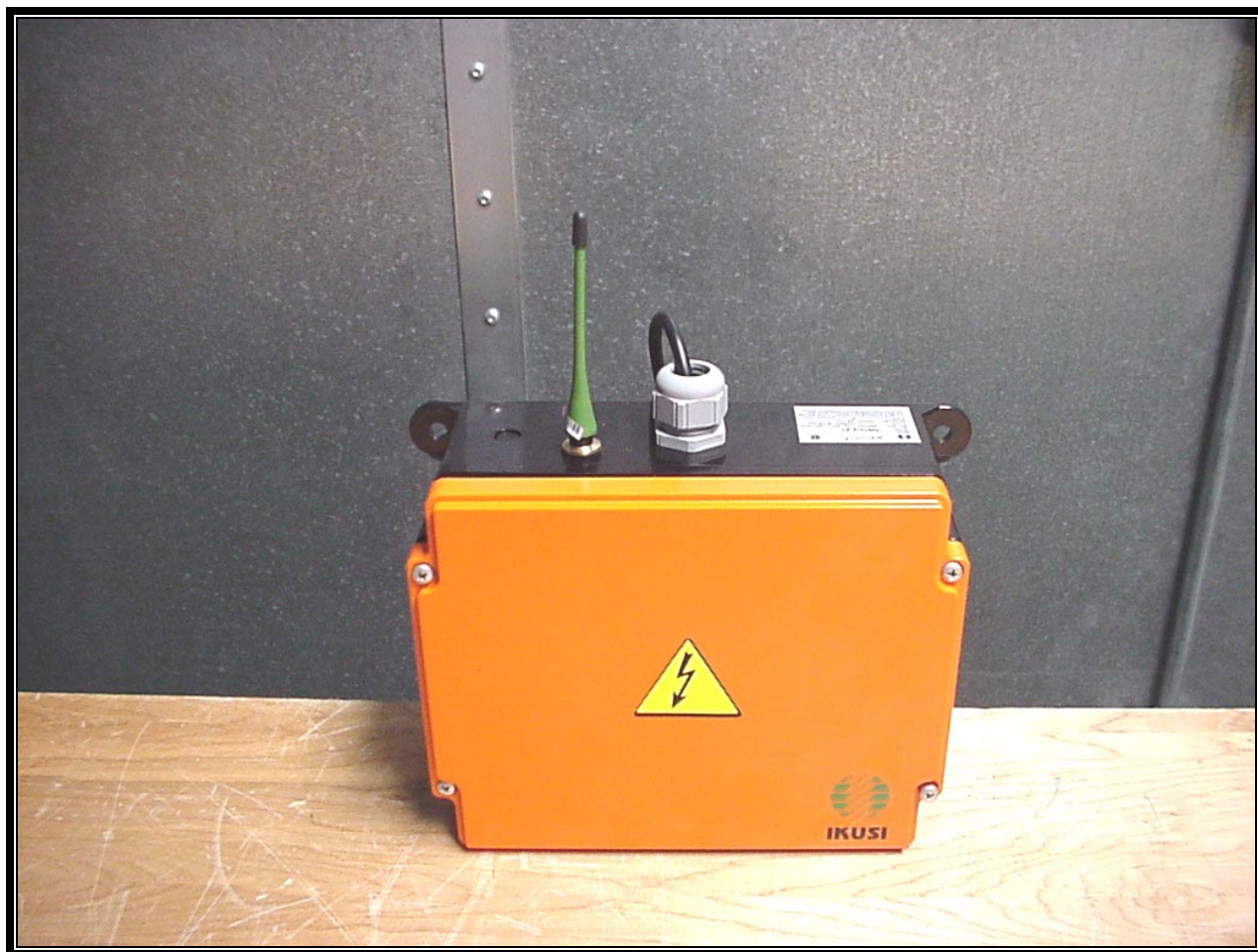
PHOTOGRAPH 3: CONDUCTED EMISSION FRONT VIEW; TM70/2.21
