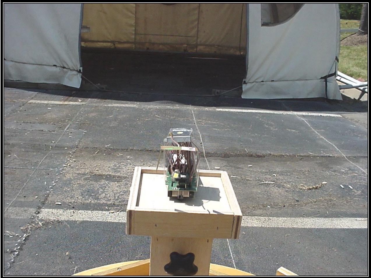
PHOTOGRAPH 5: RADIATED EMISSION FRONT VIEW WORST CASE CONFIGURATION
