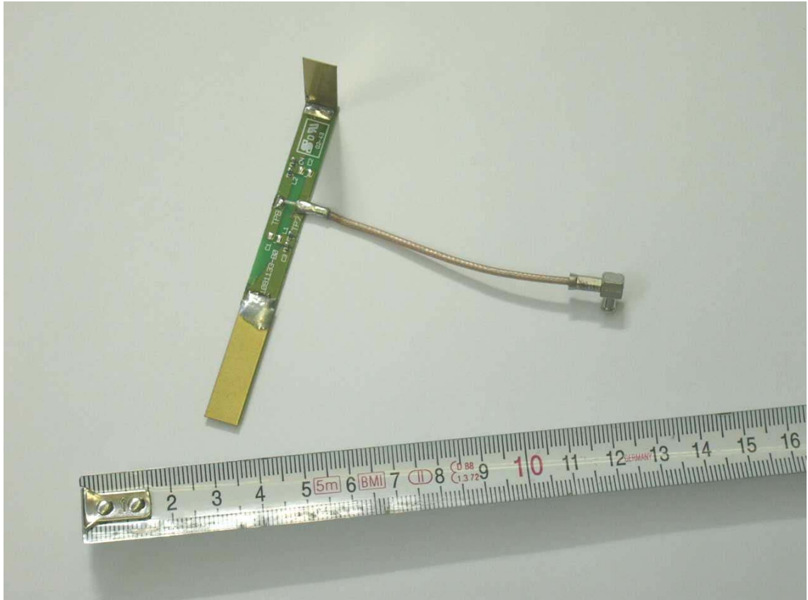
Figure 8. Internal Antenna Model AKR. Low Power. Code 2303721.jpg
