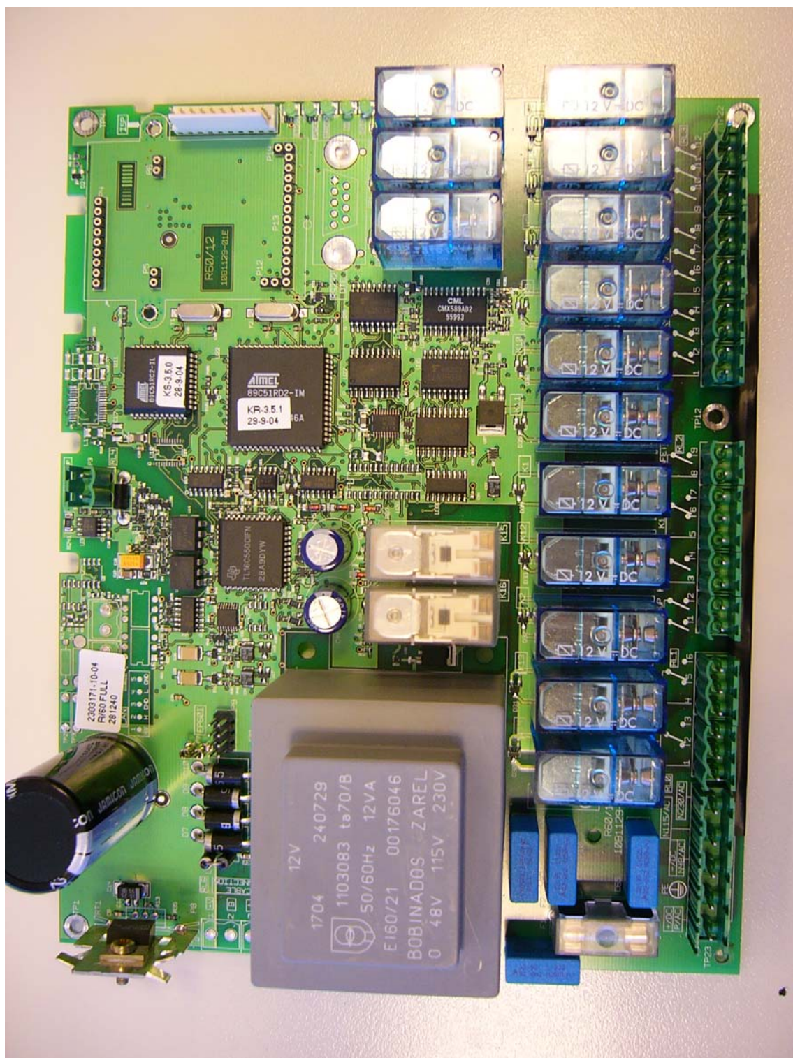
Figure 2. R6012K. Top view of PCB.JPG
