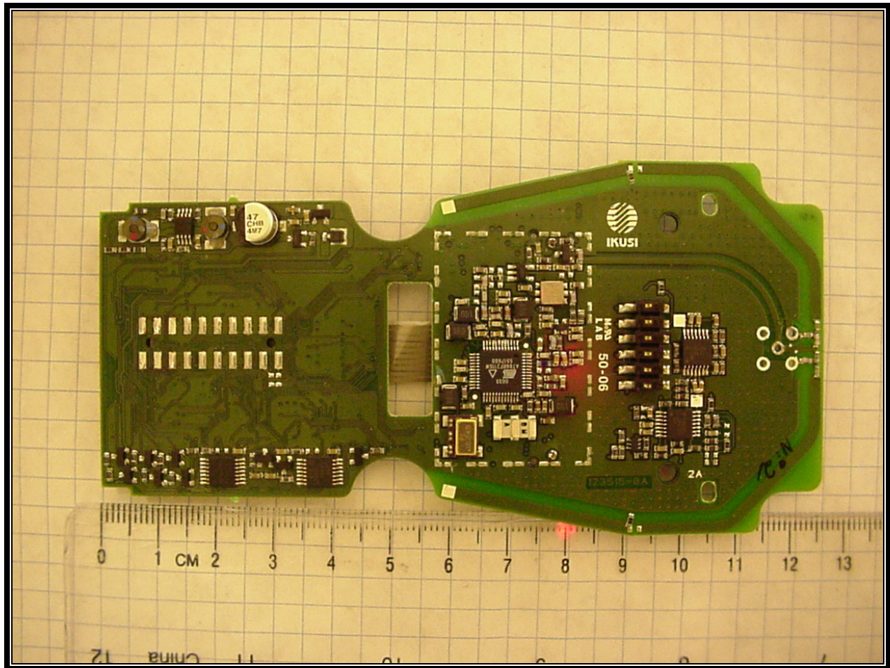
Photograph 8: PCB Back with Shield Removed
