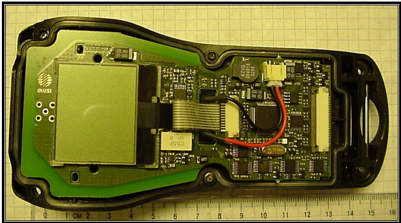
Photograph 6: PCB Front
