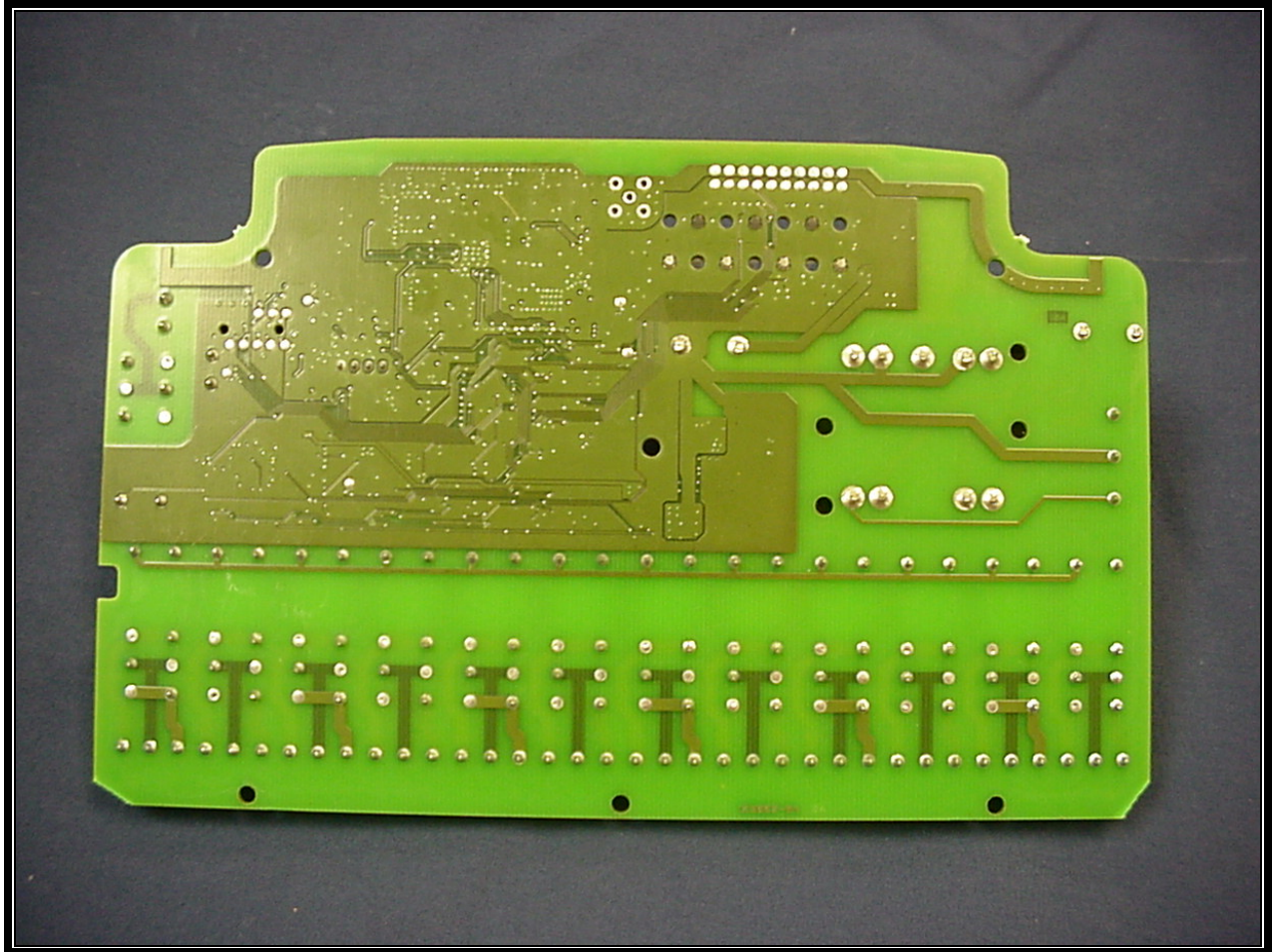
Photograph 11: PCB Bottom
