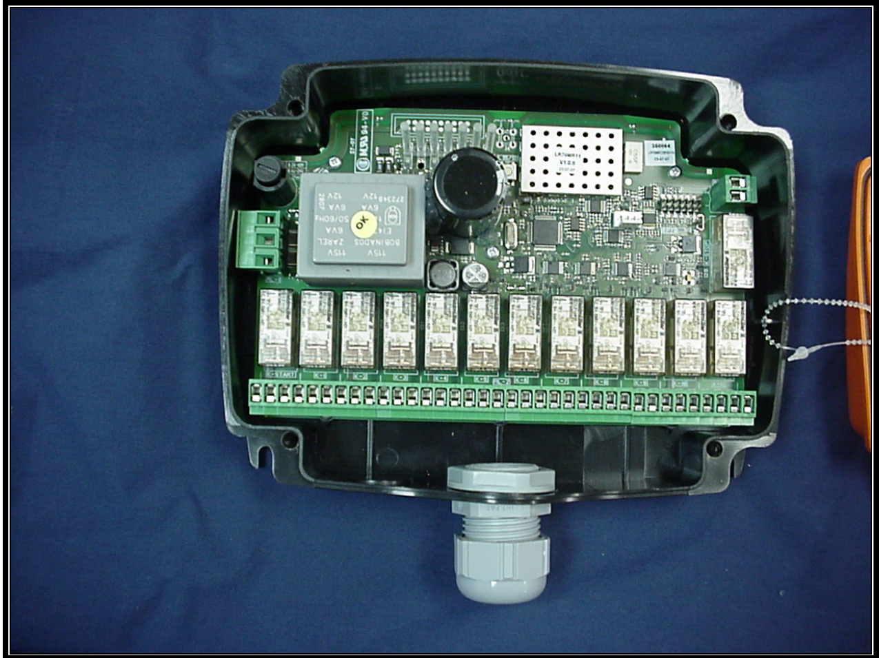
Photograph 8: PCB Mounted in Case
