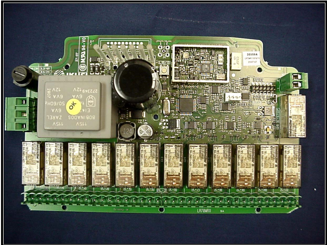
Photograph 10: PCB Top without Shield
