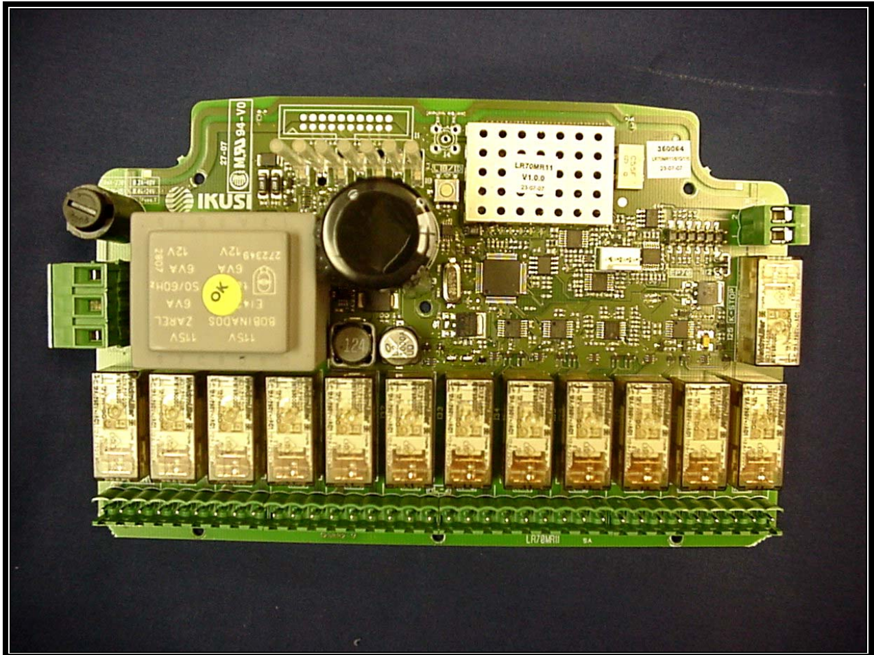
Photograph 9: PCB Top with Shield
