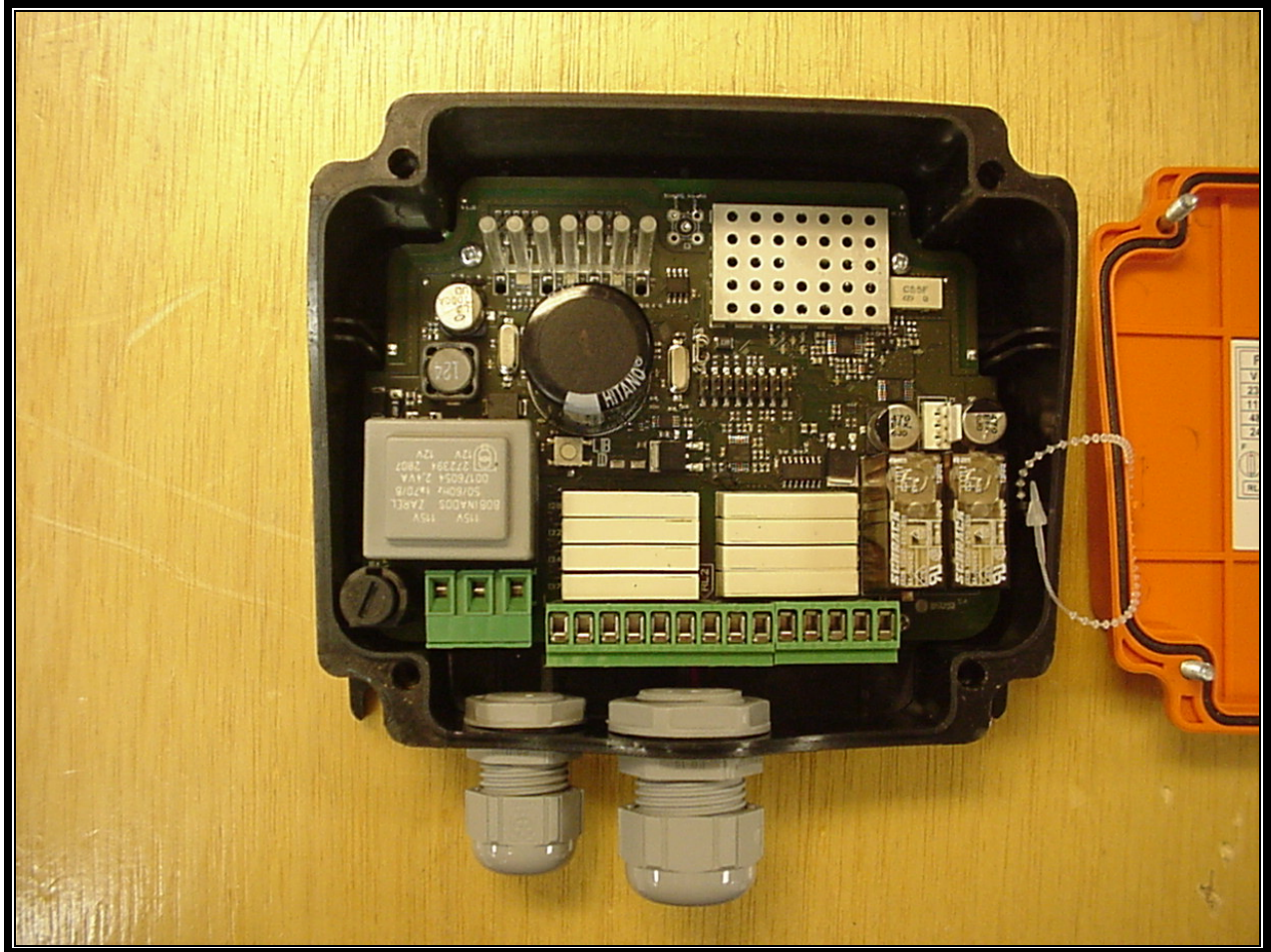
Photograph 10: PCB Mounted in Case
