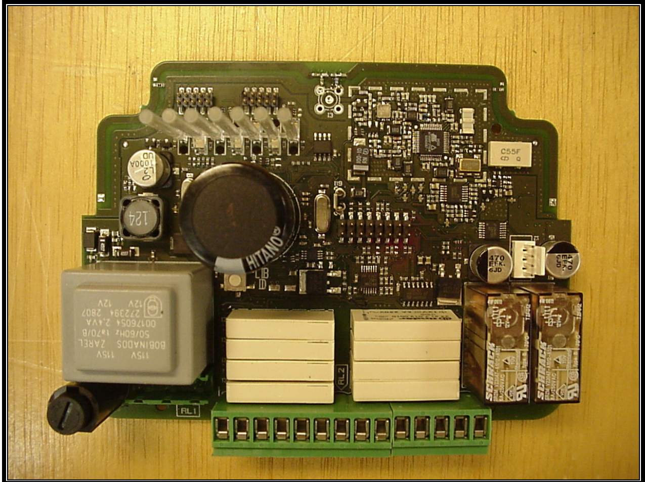
Photograph 12: PCB Top without Shield
