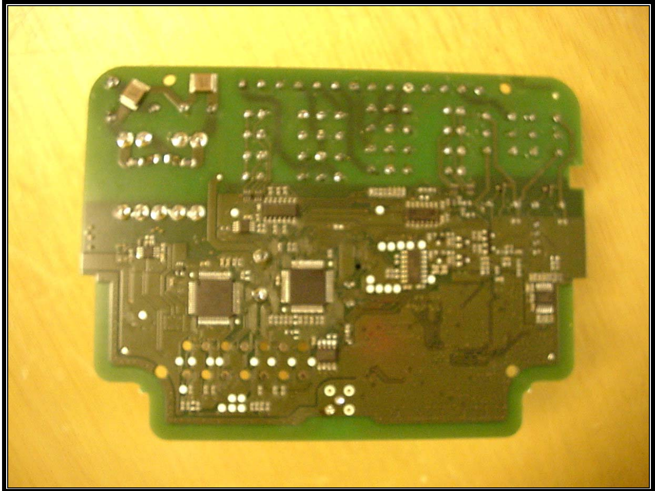
Photograph 13: PCB Bottom
