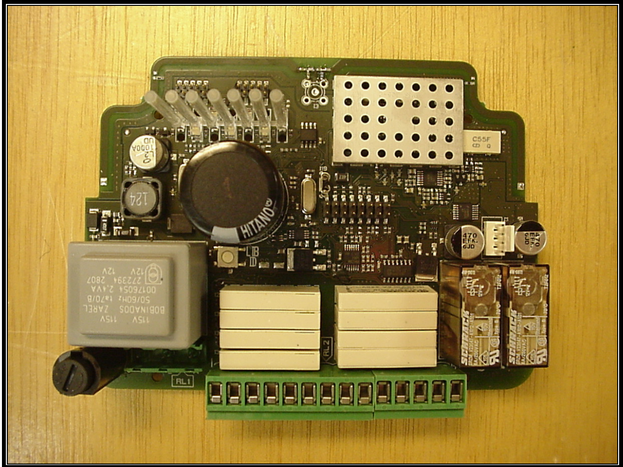
Photograph 11: PCB Top with Shield
