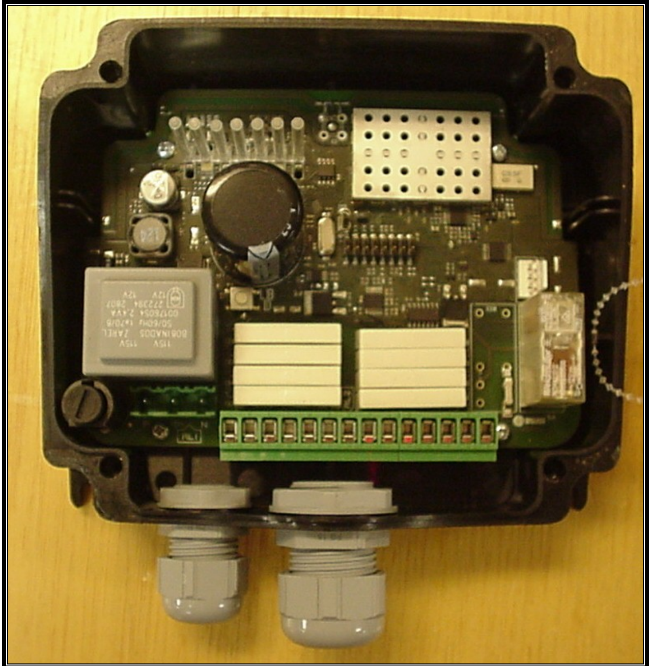
Photograph 9: PCB Mounted in Case
