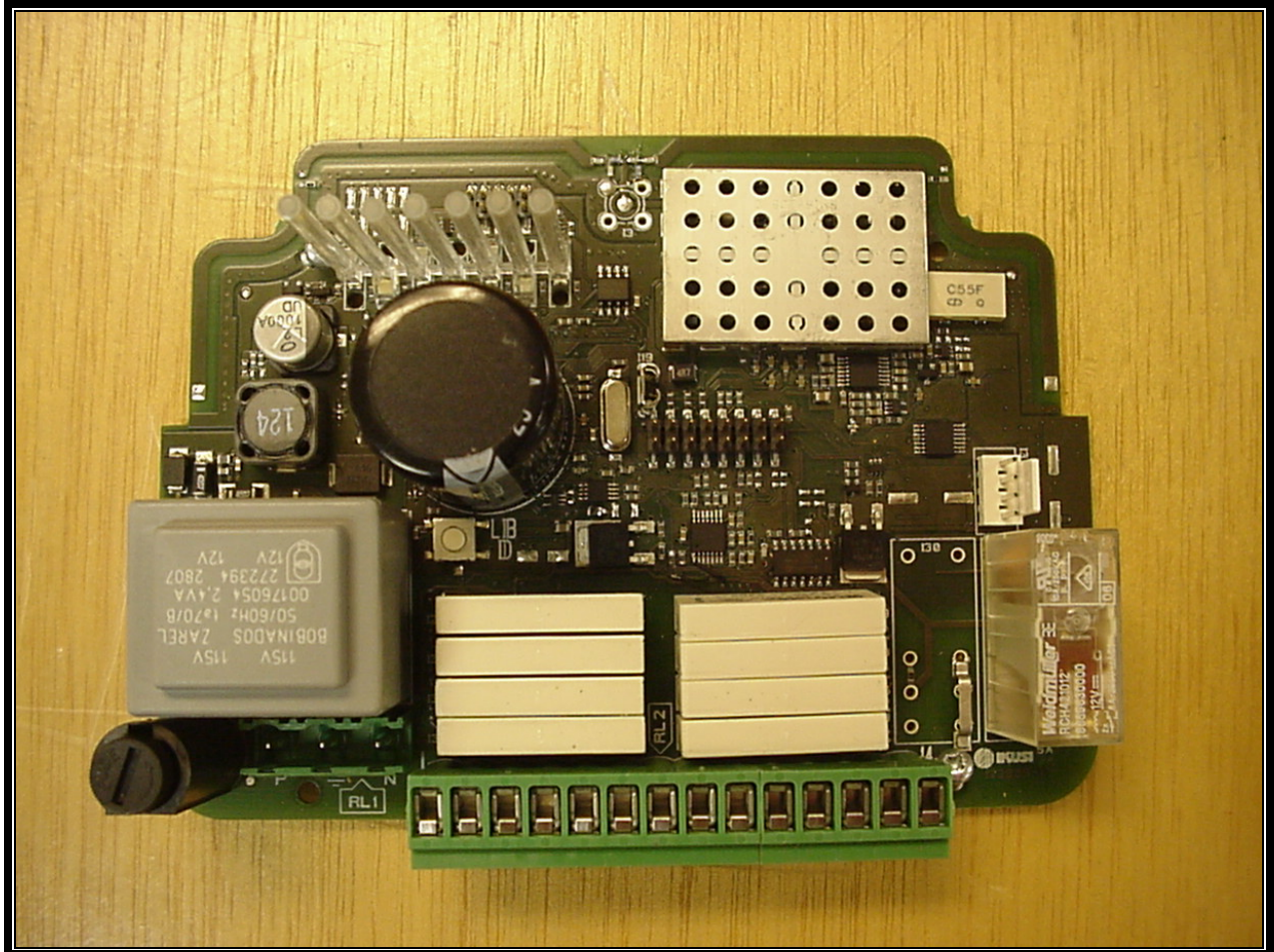
Photograph 10: PCB Top with Shield
