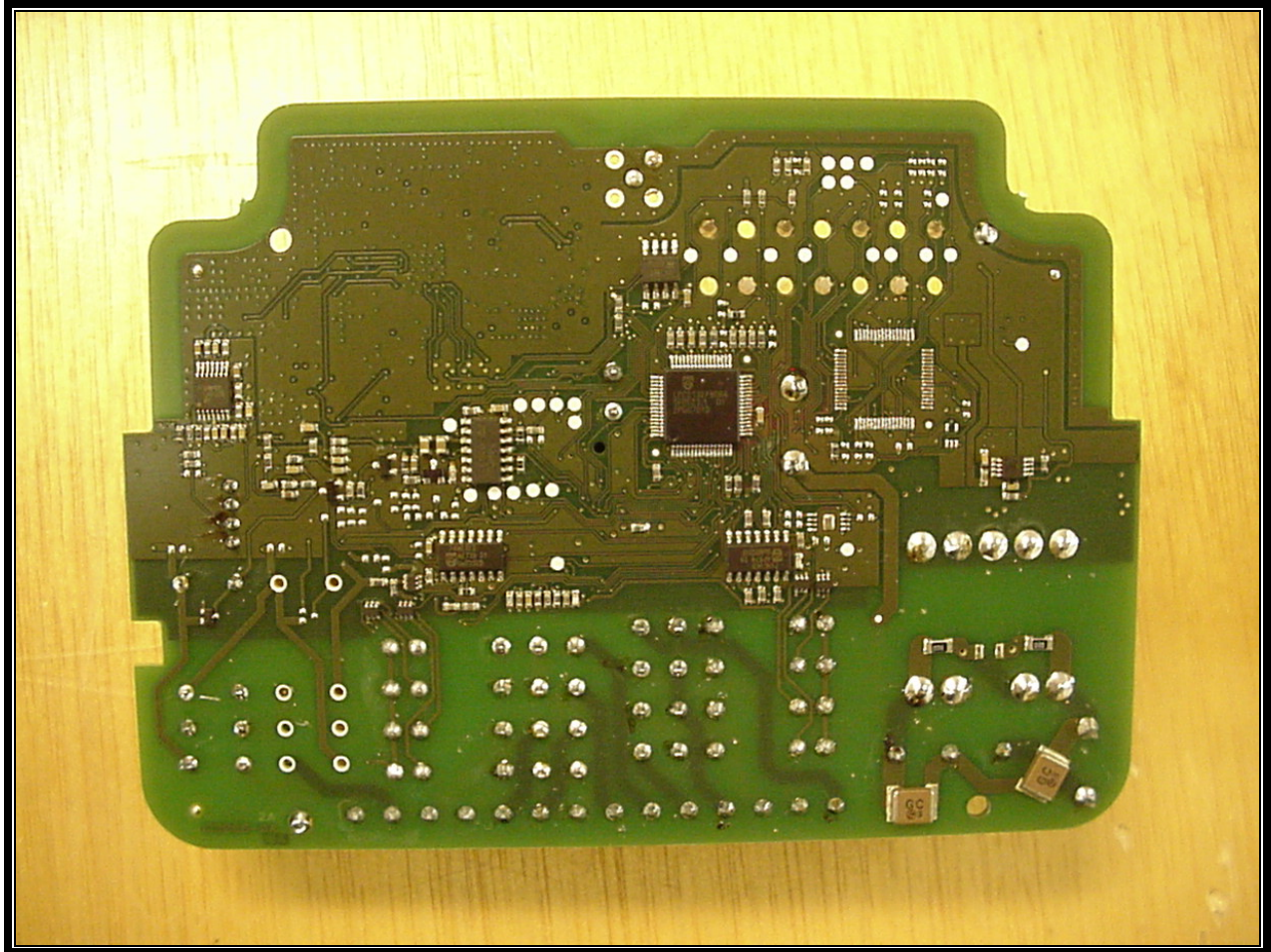
Photograph 12: PCB Bottom
