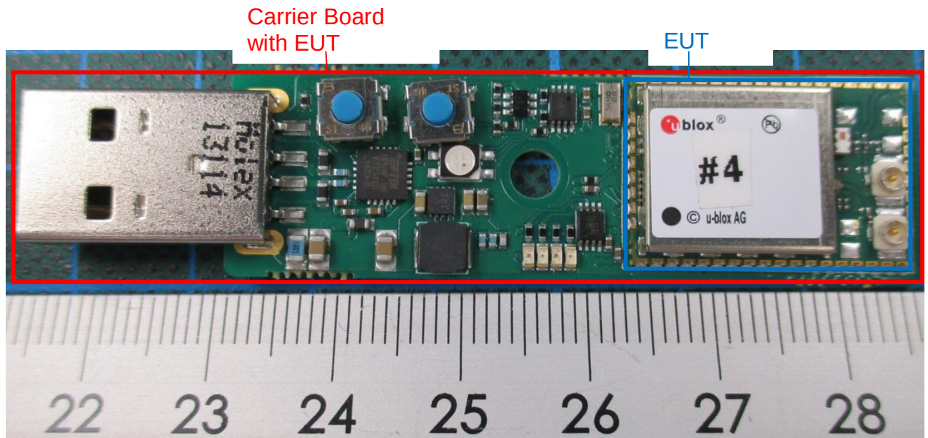
151496_01.jpg: Carrier Board + EUT – Top View (Odin-W260)
