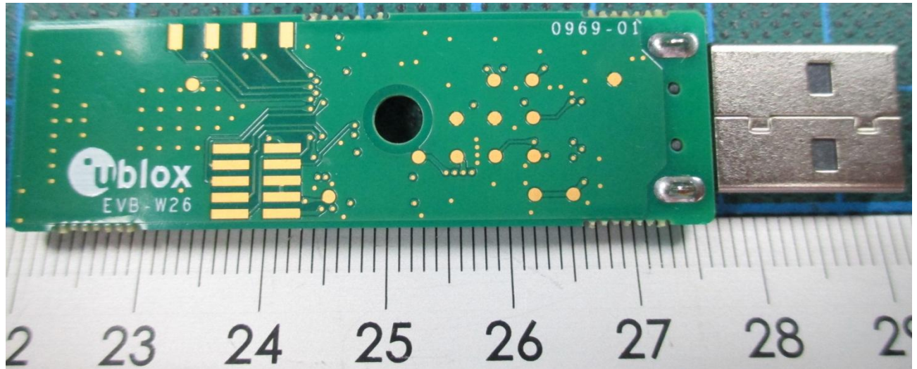
151496_02.jpg: Carrier Board – Bottom View (Odin-W260)
