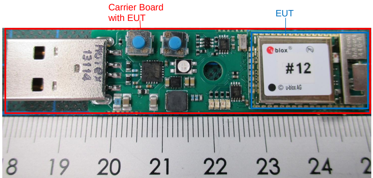
151496_06.jpg: Carrier Board + EUT – Top View (Odin-W262)
