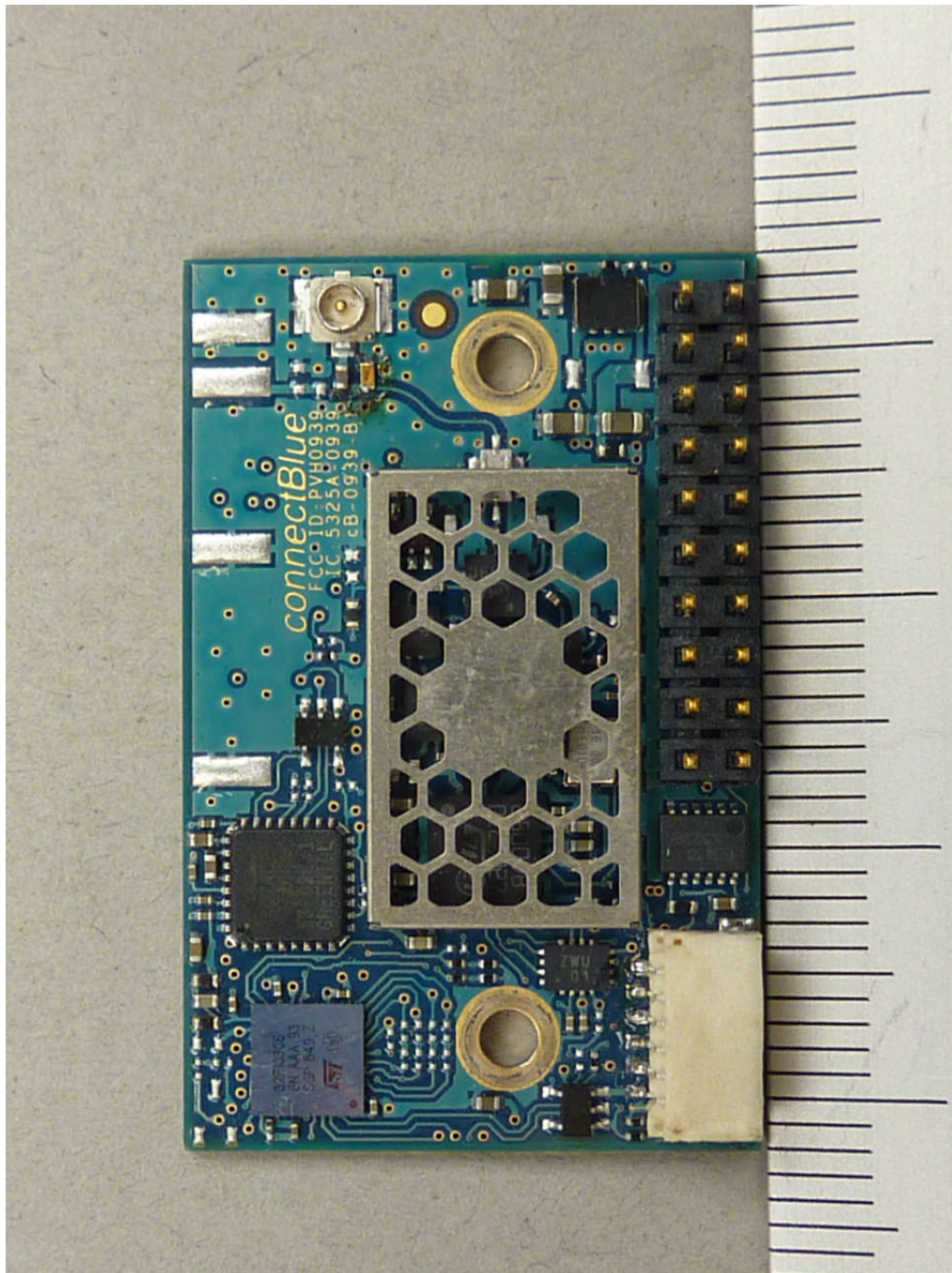
112117_g.JPG: cB-0939, PCB, top view
