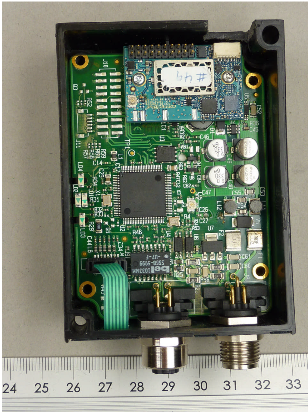
112117_d.JPG: cB-0939 mounted on the cB-0924-02 (EPA)
