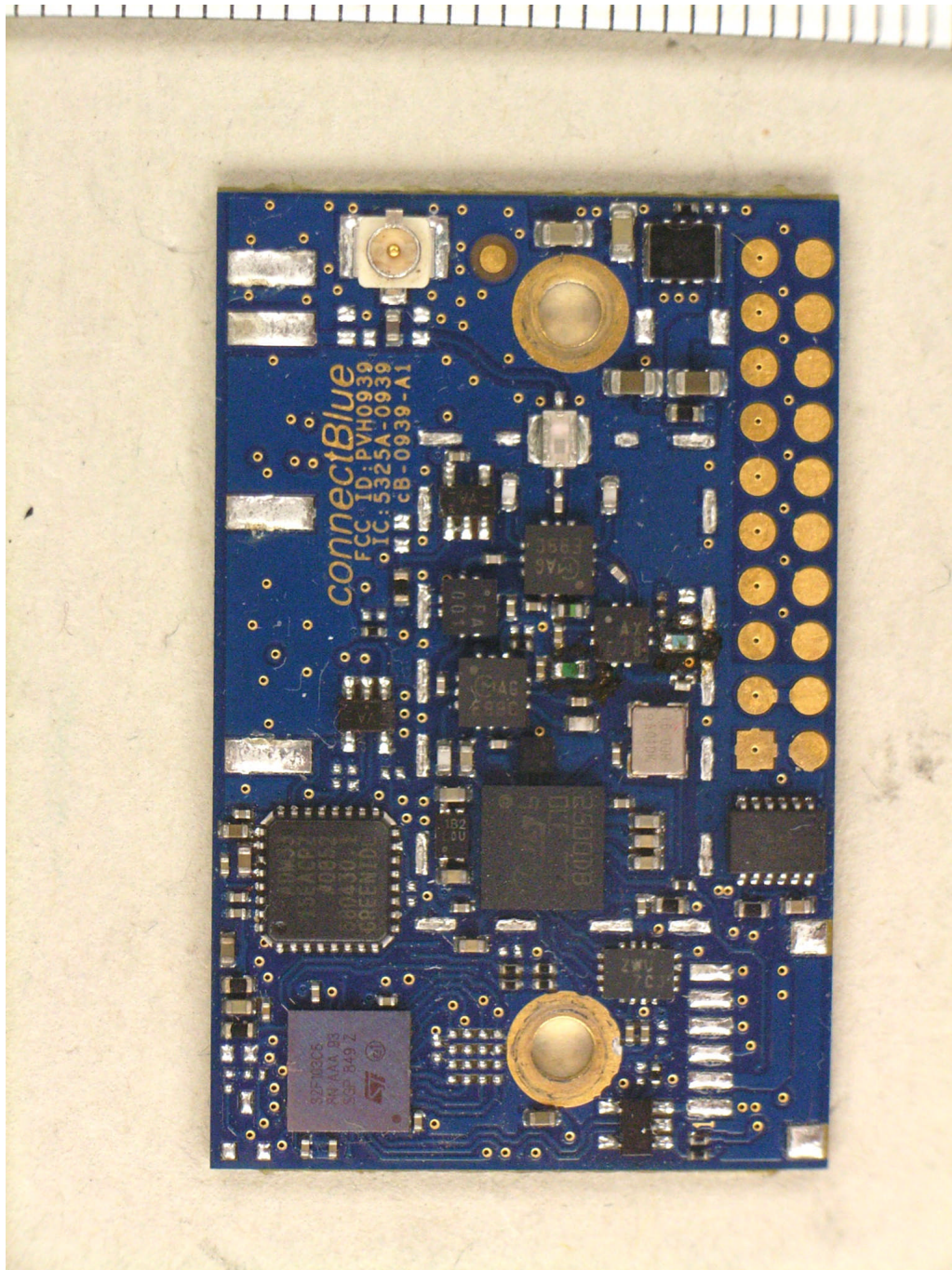
112117_h.JPG: cB-0939, PCB, top view, shielding removed
