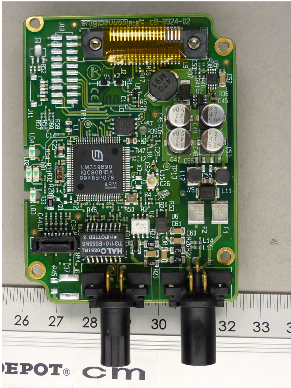
112117_i.JPG: cB-0924-02 (EPA), top view, cB-0939 removed
