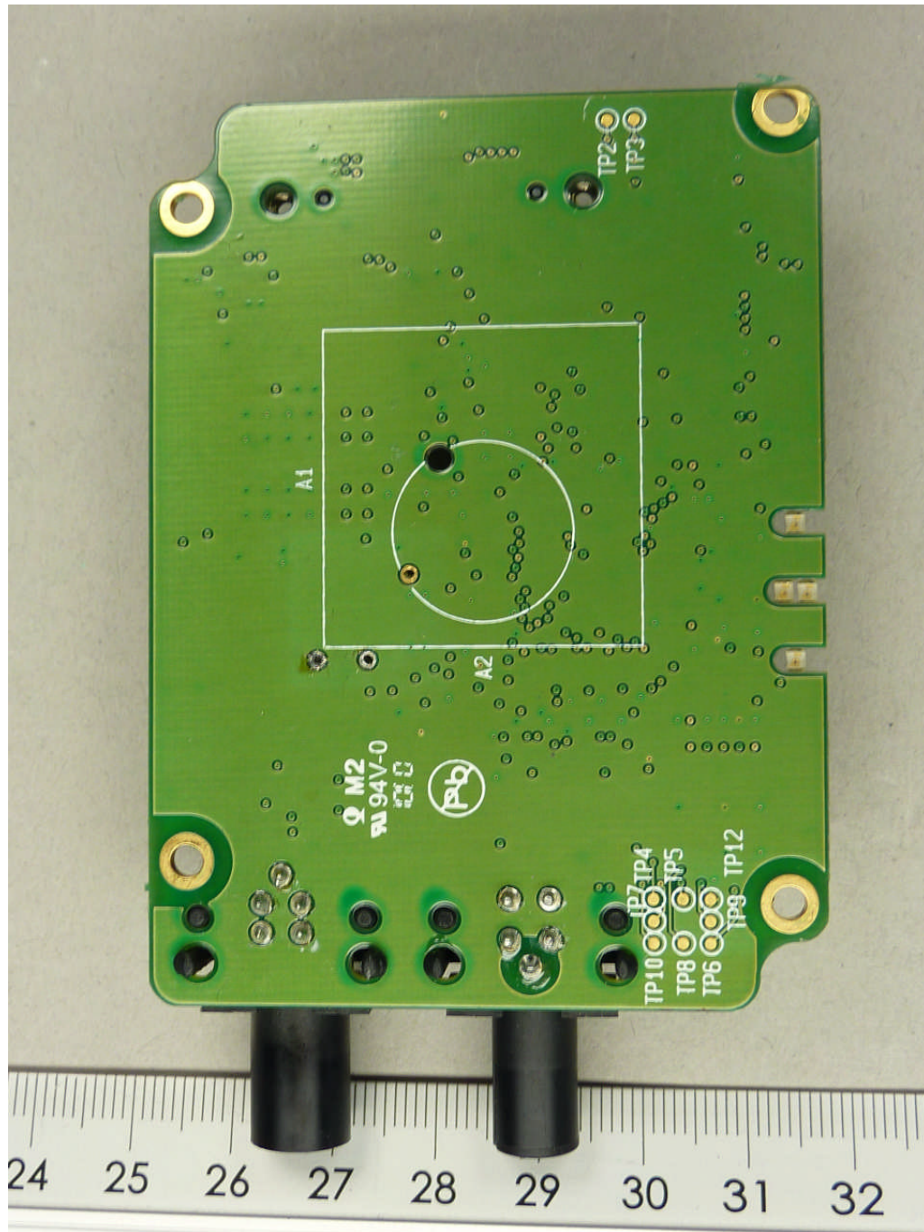
112117_j.JPG: cB-0924-02, bottom view, antenna removed
