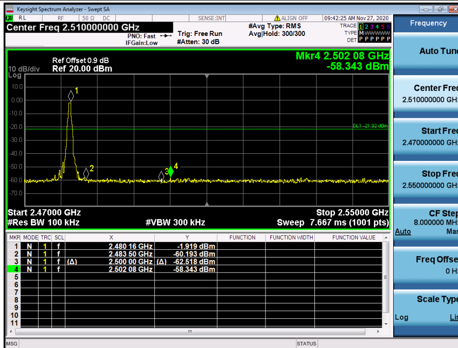
DH5_Ant1_High_2480
