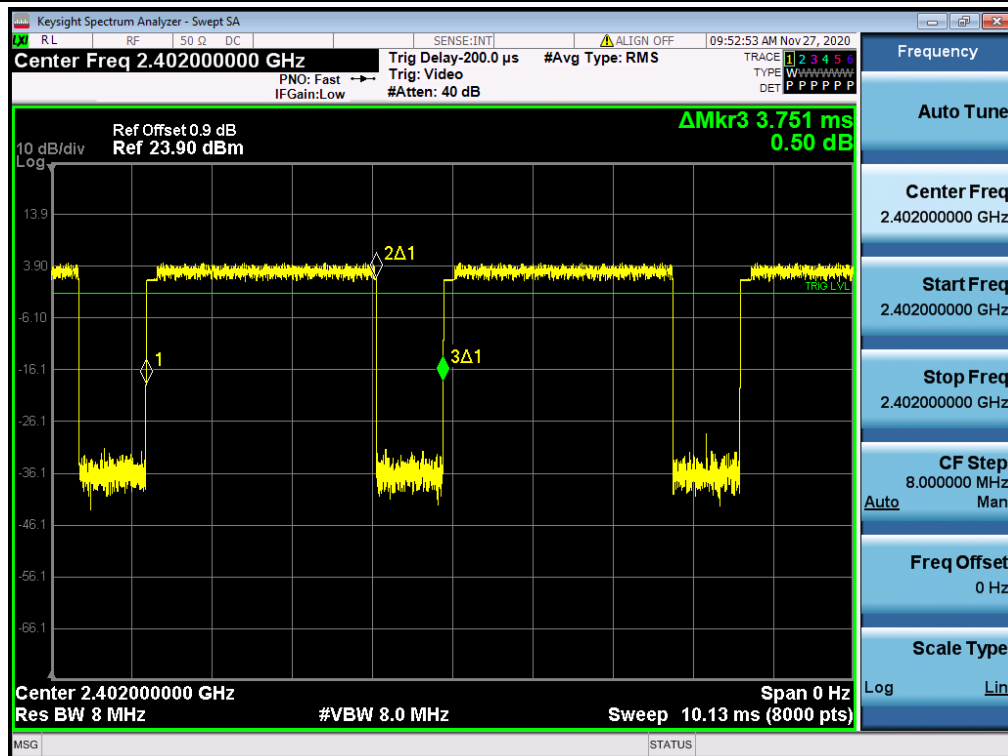
3DH5_Ant1_2402
