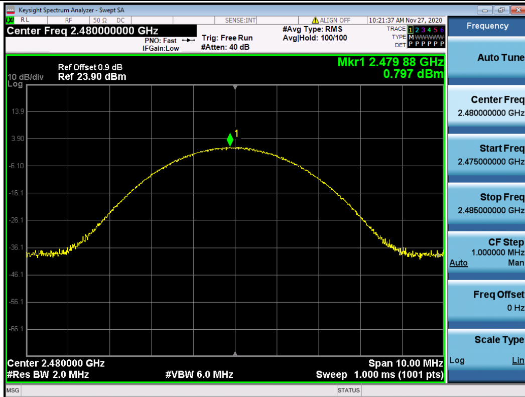
3DH5_Ant1_2480
