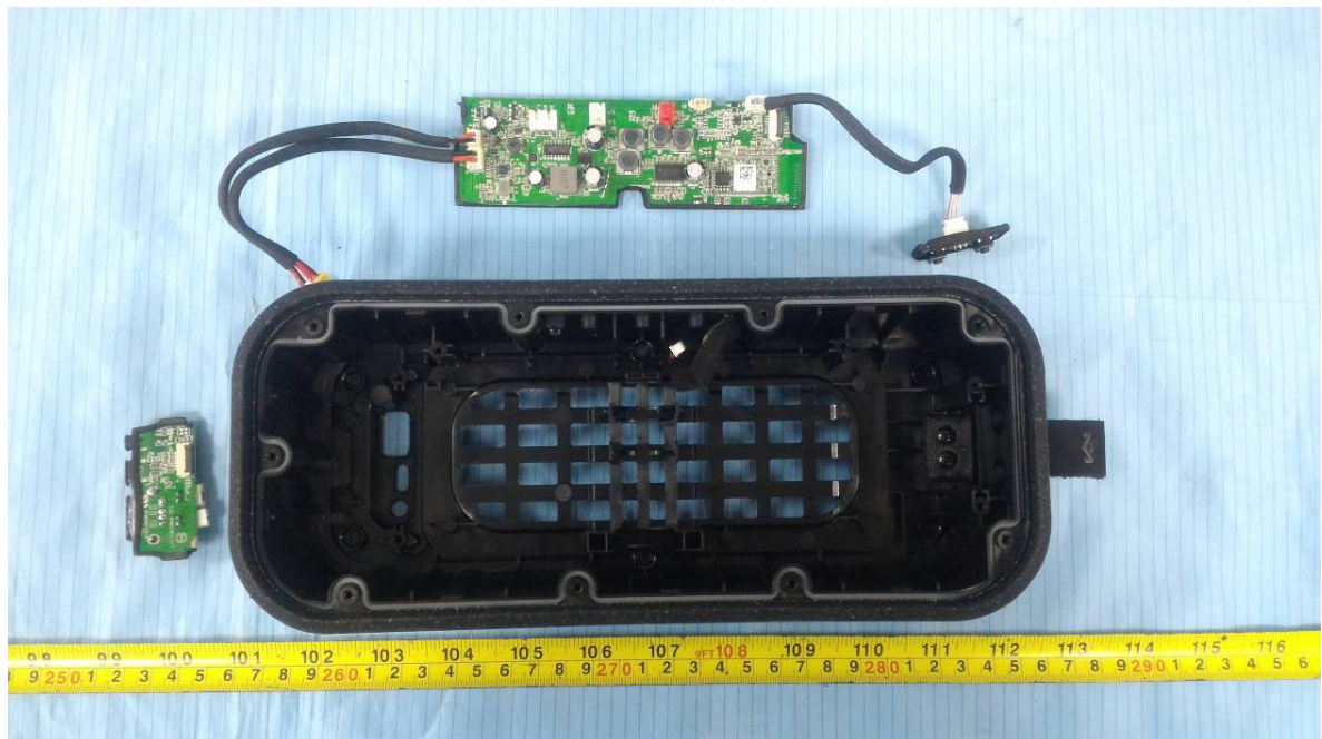
EUT – Cover off View (6)
