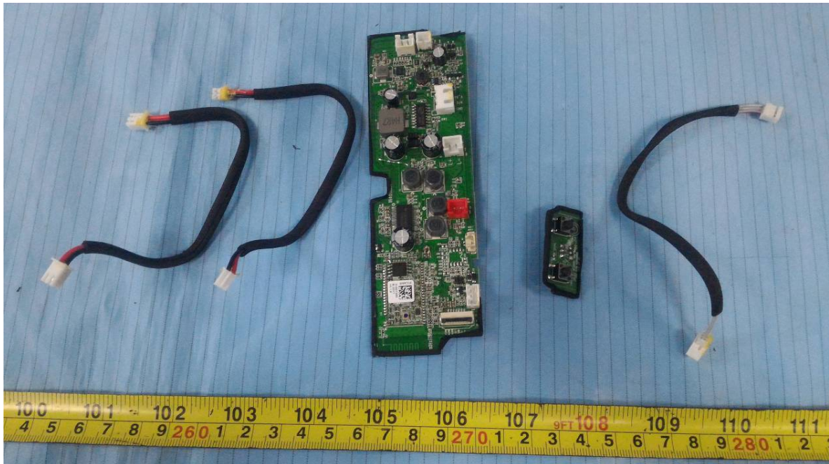
EUT – Cover off View (7)
