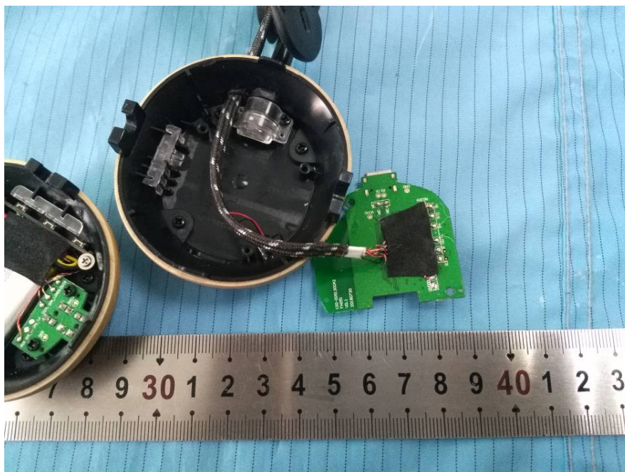
EUT – Left Part Cover off View
