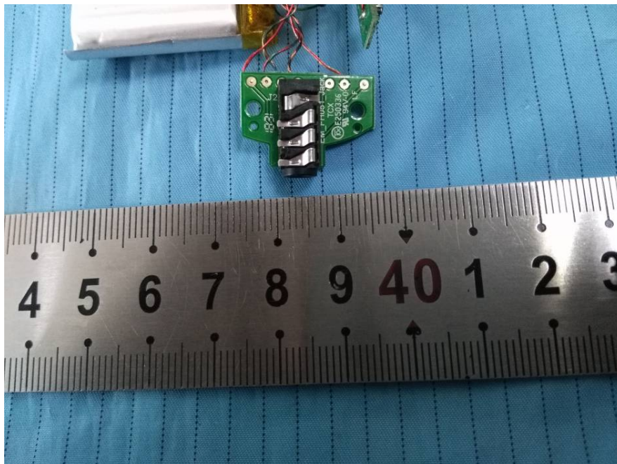
EUT – Audio Part Board Bottom View
