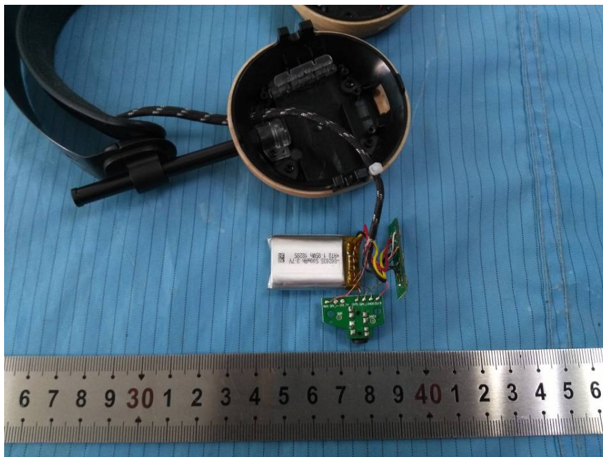
EUT – Right Part Cover off View
