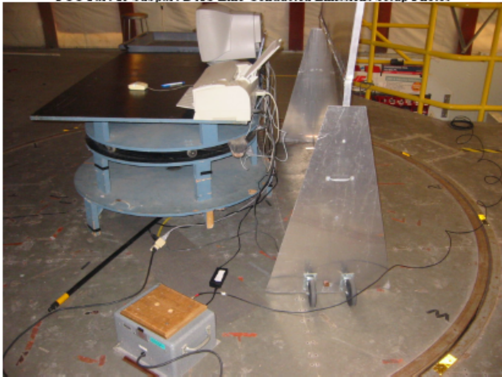
FCC Part 15 Subpart B AC Line-Conducted Emissions Setup Photos
