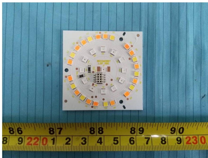
EUT – LED Board Front View
