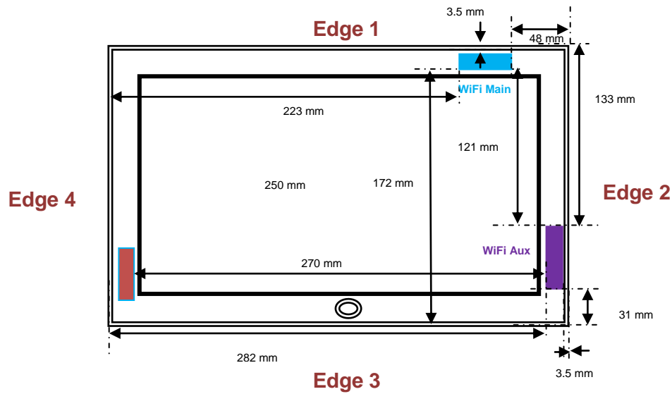
Front View
