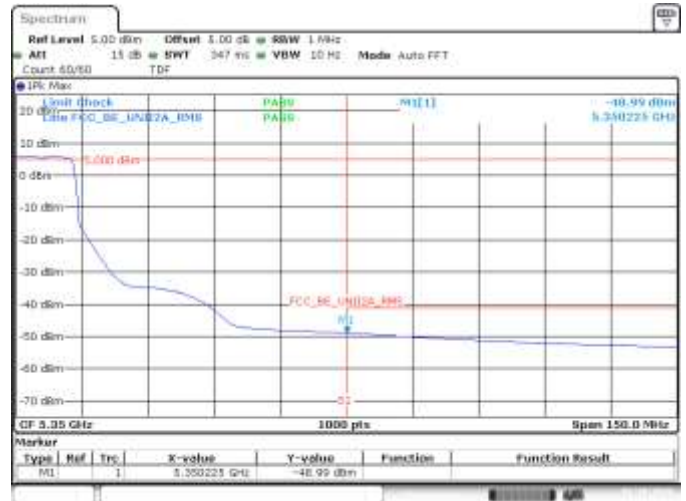
MIMO A, 802.11n20, HT8, CH54, BE High RMS
