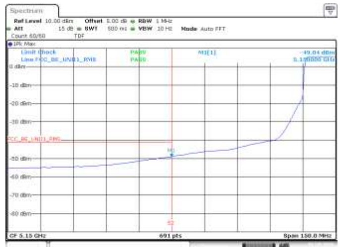
MIMO B, 802.11ax40, HE0, CH38, BE Low, RMS
