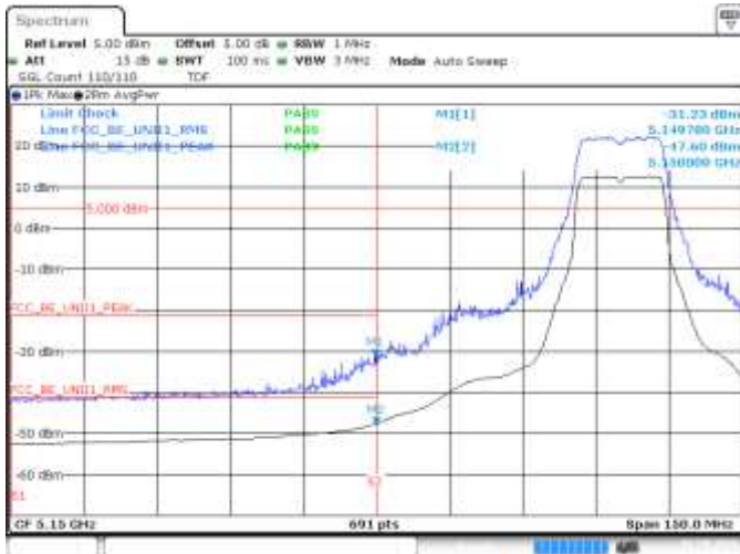
MIMO B, 802.11n20, HT8, CH40, BE Low, RMS, Peak
