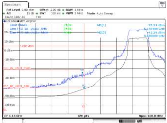
SISO B, 802.11n20, HT0, CH40, BE Low, RMS, Peak
