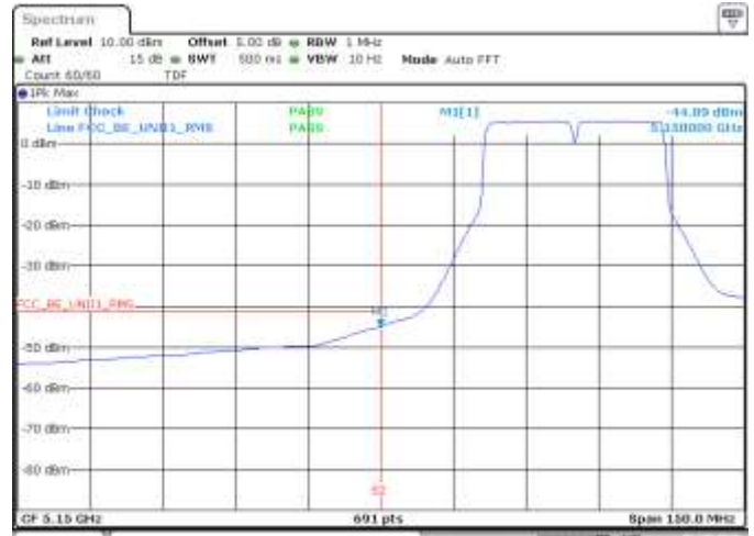
MIMO B, 802.11n20, HT8, CH40, BE Low, RMS
