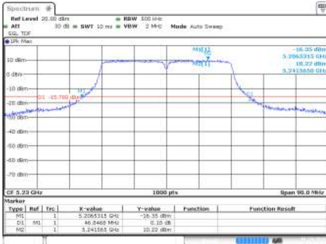
MIMO A, CH46, 802.11n40, HT0, 26dB BW
