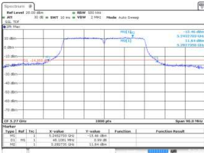
SISO B, CH54, 802.11n40, HT0, 26dB BW
