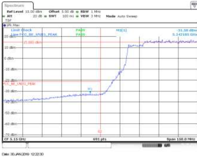
MIMO B, 802.11ax80, HE0, CH42, BE Low, Peak
