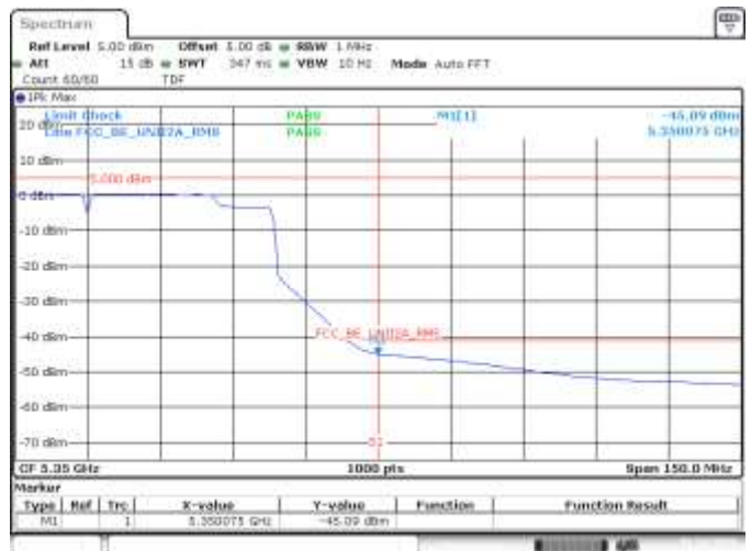
SISO B, 802.11ac80, VHT0, CH58, BE High RMS
