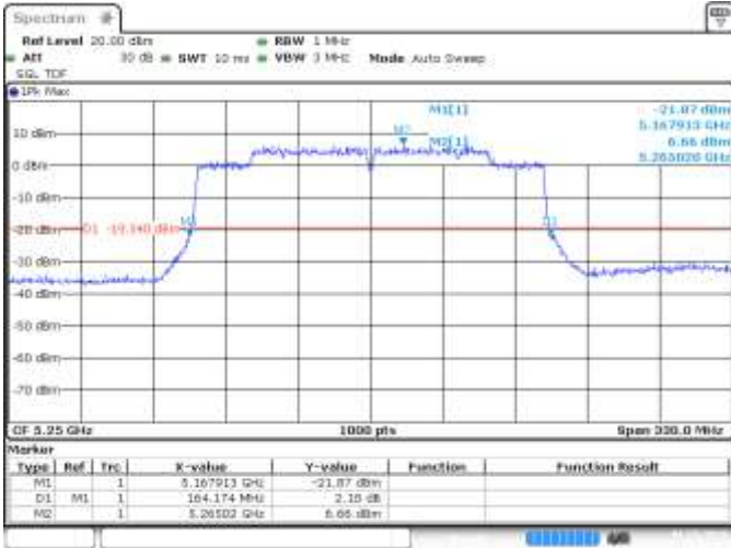
SISO B, CH50, 802.11ax160, HE0, 26dB BW
