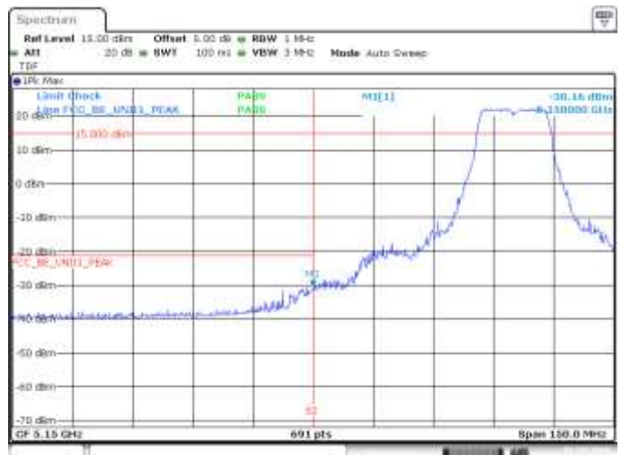
MIMO B, 802.11n20, HT8, CH36, BE Low, RMS, Peak
