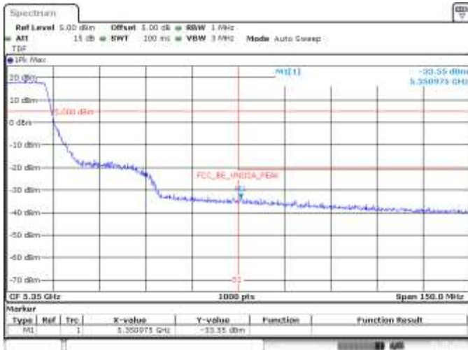
MIMO A, 802.11n20, HT8, CH54, BE High Peak
