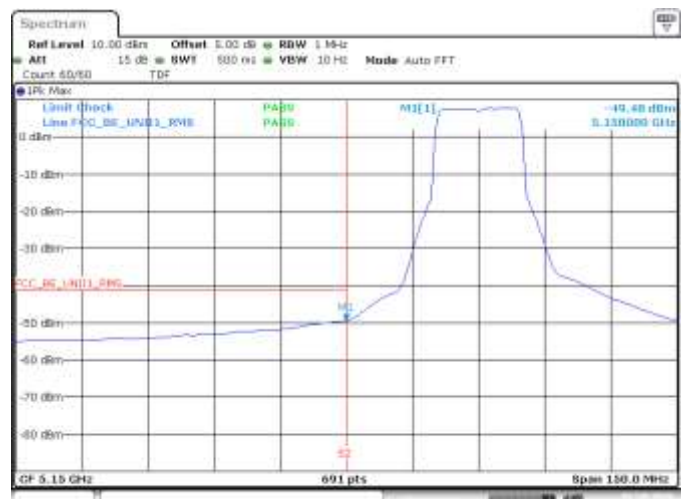
MIMO A, 802.11ax20, HE0, CH40, BE Low, RMS
