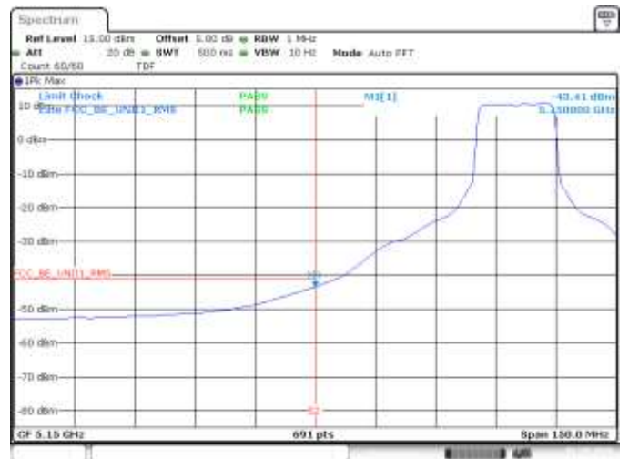
SISO B, 802.11ax20, HE0, CH36, BE Low, RMS
