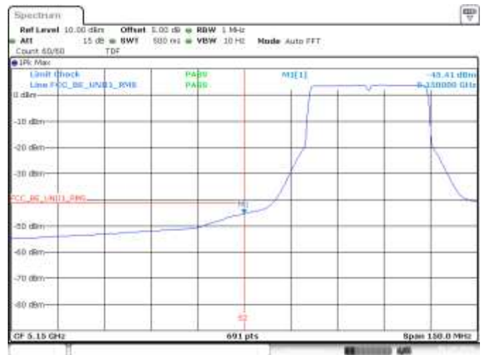
SISO B, 802.11ax40, HE0, CH46, BE Low, RMS
