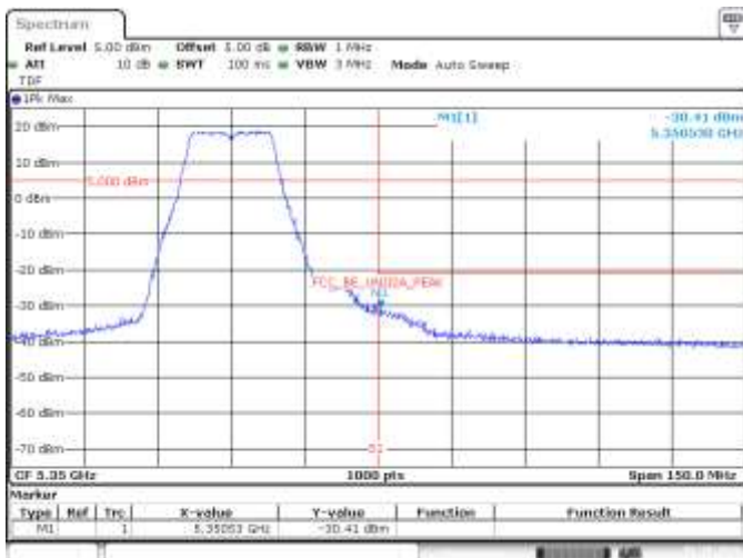
MIMO A, 802.11n20, HT8, CH62, BE High Peak
