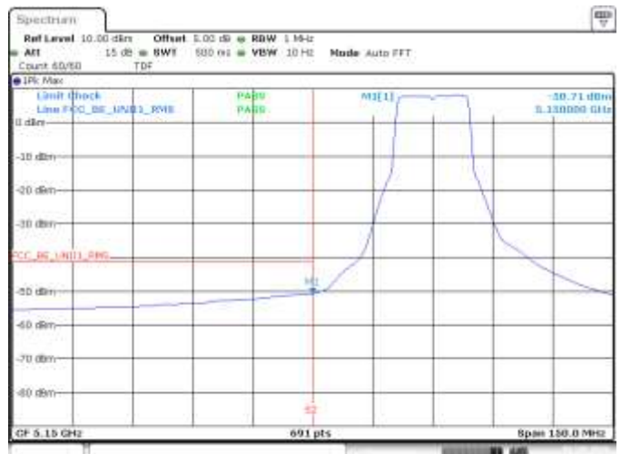
MIMO A, 802.11n20, HT8, CH36, BE Low, Peak
