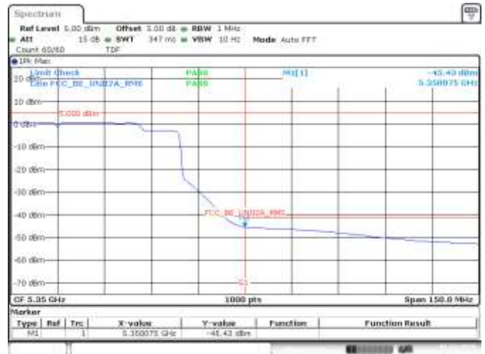
MIMO A, 802.11ax80, HE0, CH58, BE High RMS
