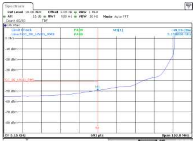
MIMO B, 802.11n40, HT8, CH38, BE Low, RMS
