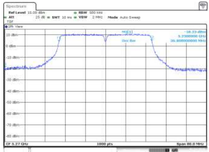
SISO B, CH54, 802.11n40, HT0, 99% BW
