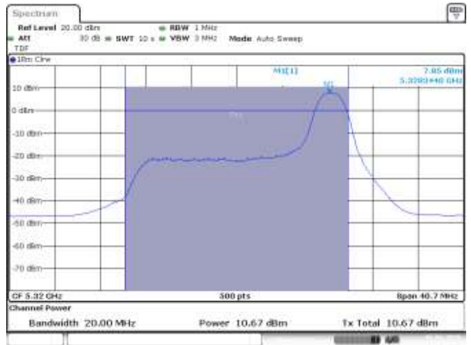
MIMO B, CH64, 802.11ax20, HE0, RU26_8
