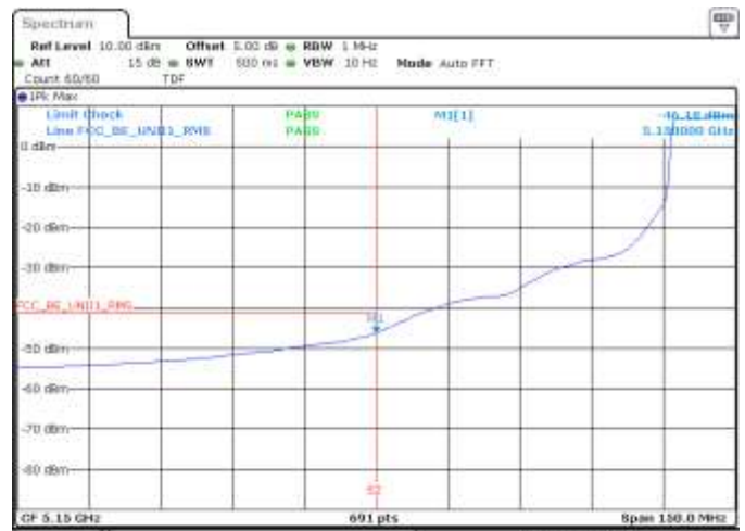
SISO A, 802.11n40, HT0, CH38, BE Low, RMS
