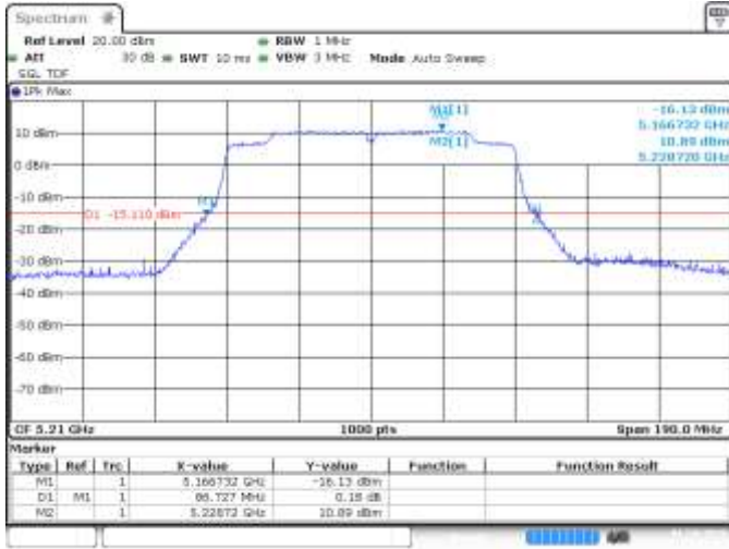
SISO A, CH42, 802.11ac80, VHT0, 26dB BW
