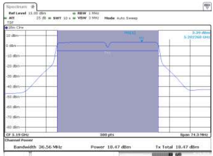
SISO B, CH38, 802.11n40, HT0
