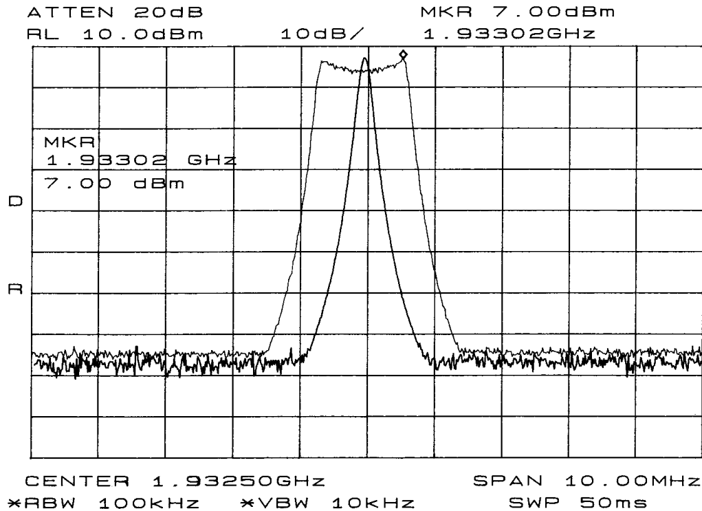
Figure 5: Occupied Bandwidth.
