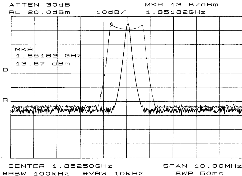
Figure 4: Occupied Bandwidth.
