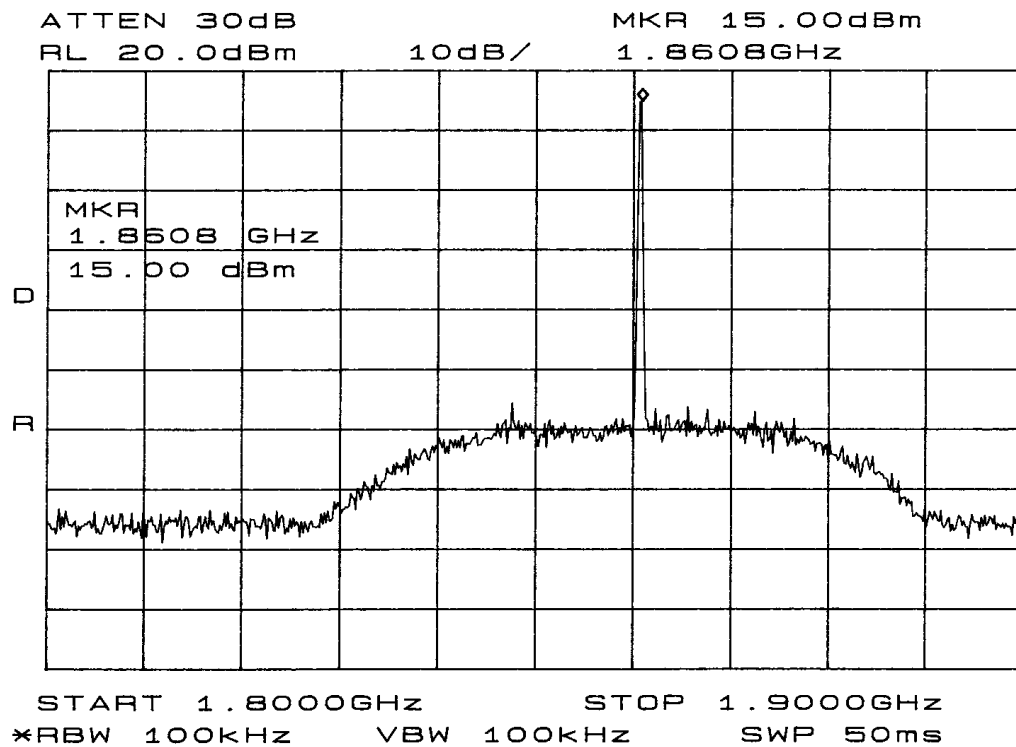
Figure 1: Uplink Power Output 1860.0 MHz.
