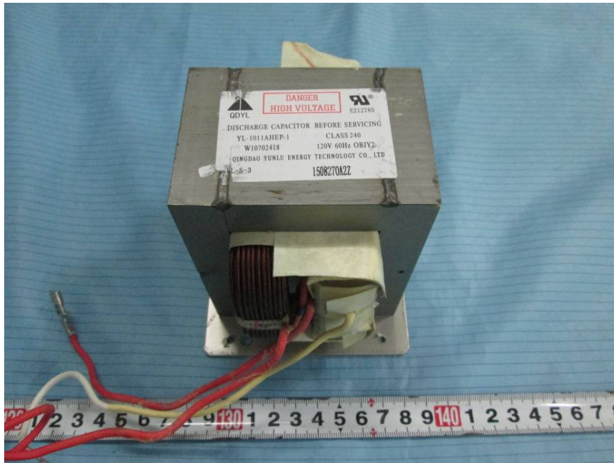
EUT – Discharge Capacitor View
