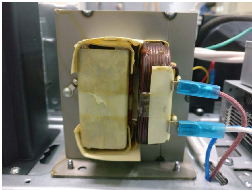
EUT –Discharge Capacitor Side View
