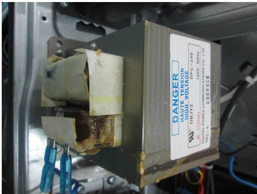
EUT –High Voltage Capacitor View
