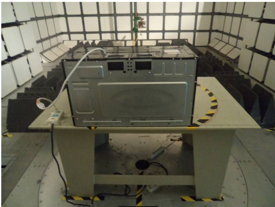
Radiated Emissions (1 GHz to 25 GHz) – Rear View
