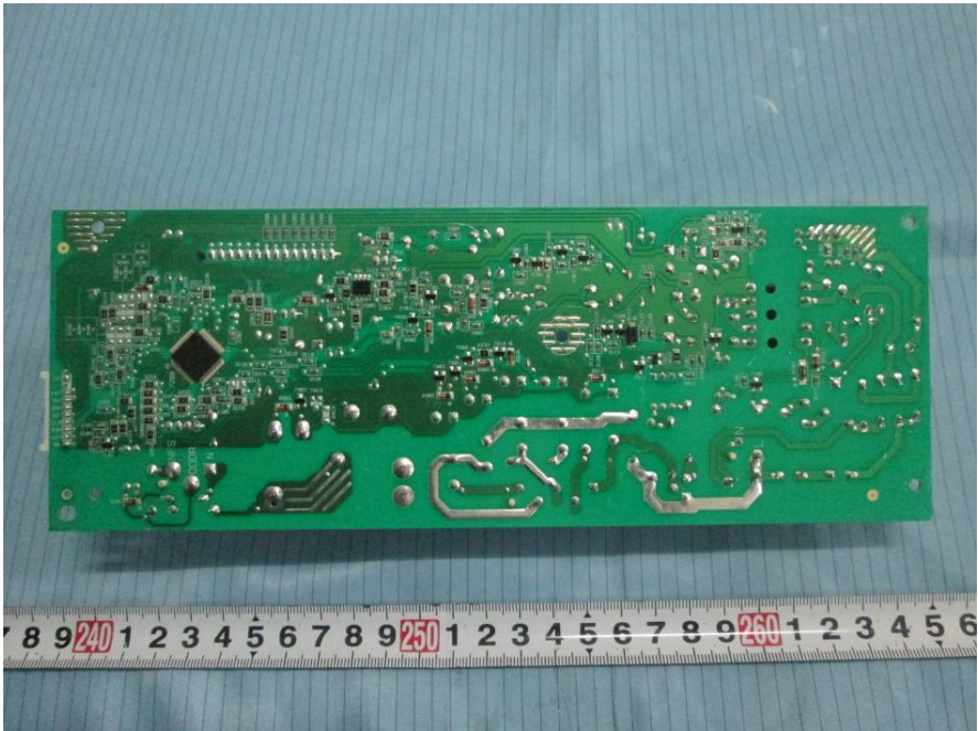
EUT – Control Pannel PCB Bottom View
