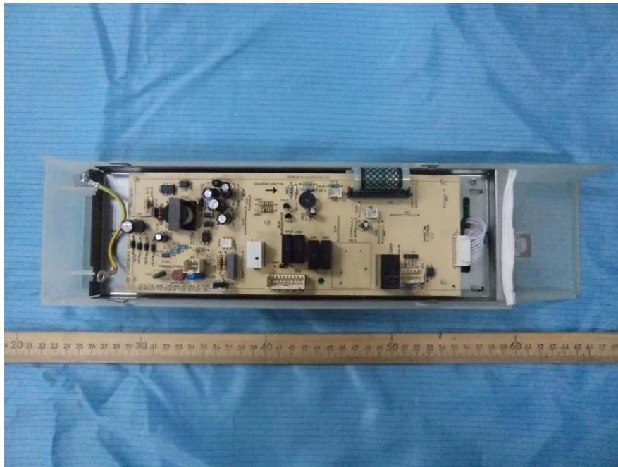
EUT – Controller Cover off View
