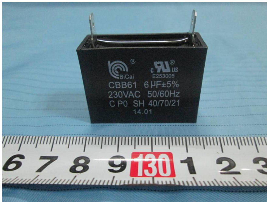
EUT –Capacitance View
