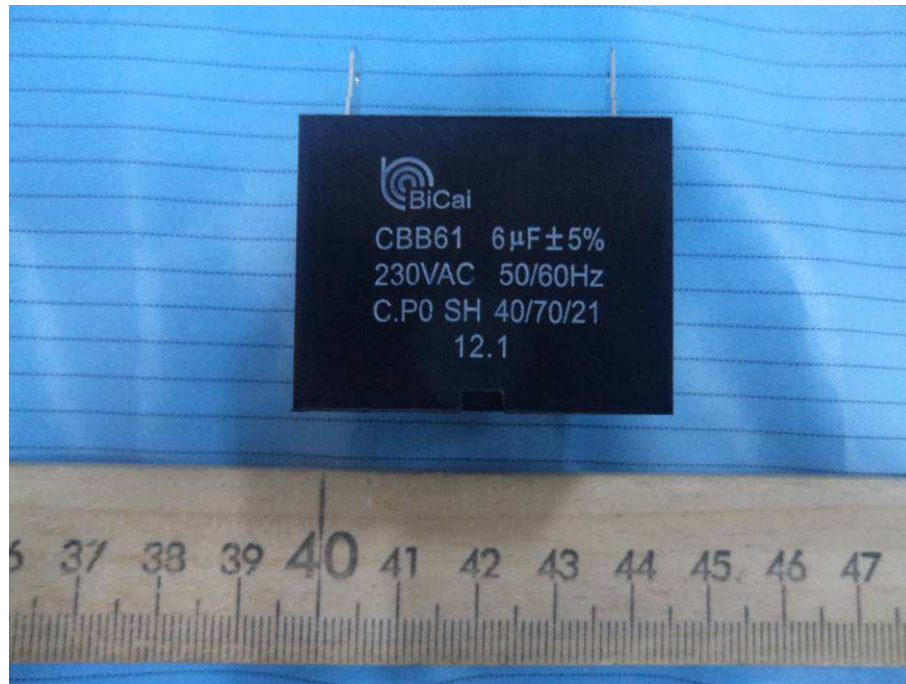
EUT – CBB61 6 \mu F Capacitor View
