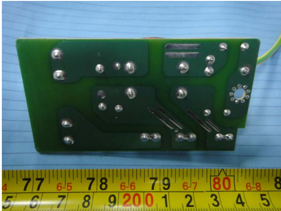
EUT – Power Board Circuit View
