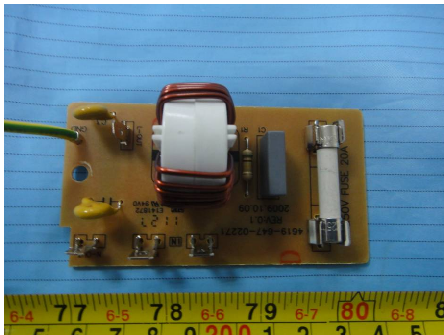
EUT – Power Board Components View
