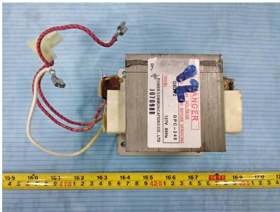
EUT – Transformer 1 front View
