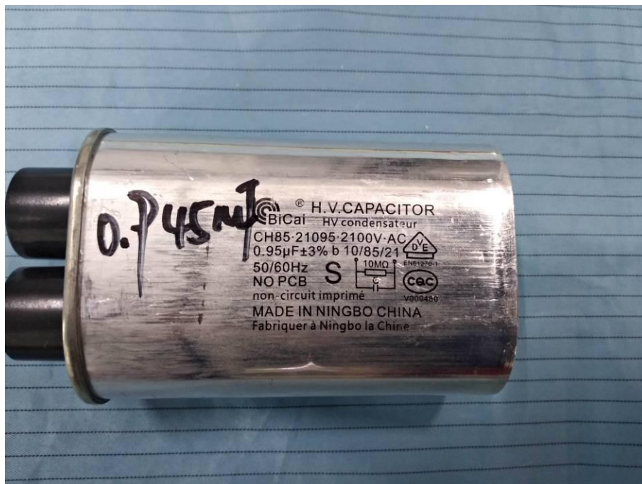
EUT – H.V. Capacitor Label View
