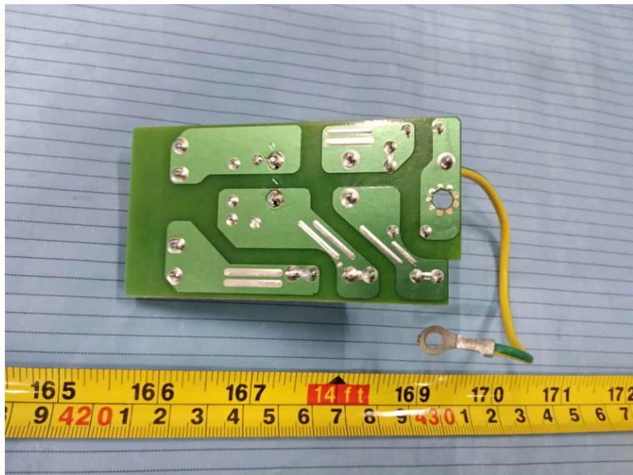
EUT – Power Supply Board Bottom View
