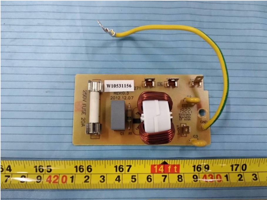
EUT – Power Supply Board Top View
