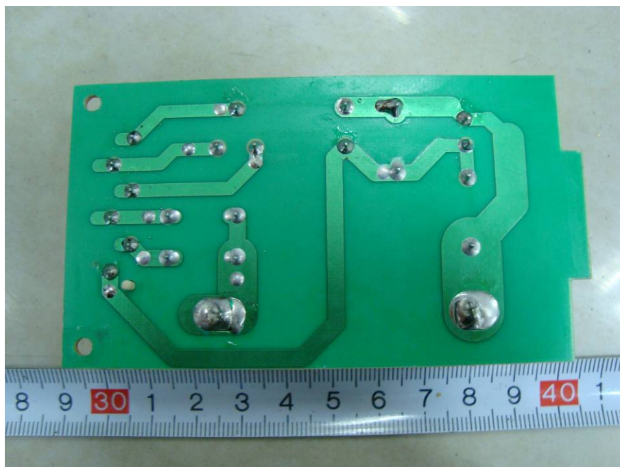
EUT – Motor Control Board Circuit View
