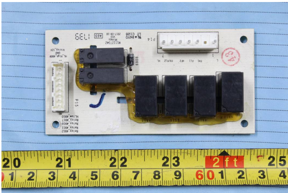
EUT – Motor-control Board Top View
