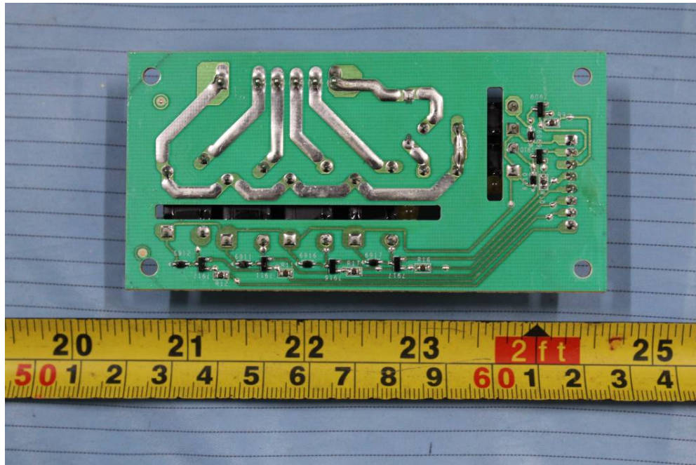
EUT – Motor-control Board Bottom View
