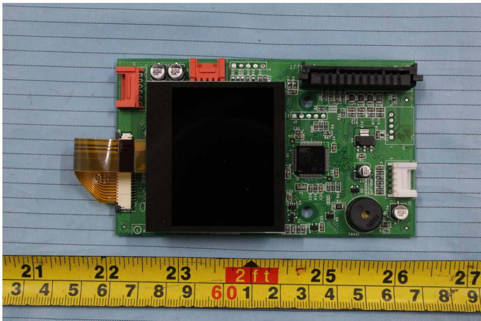
EUT – LCD Board Top View 1
