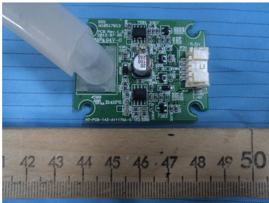
EUT – 94V-O Board Top View
