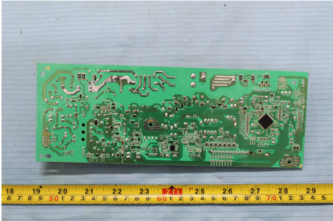
EUT – Main Board Bottom View
