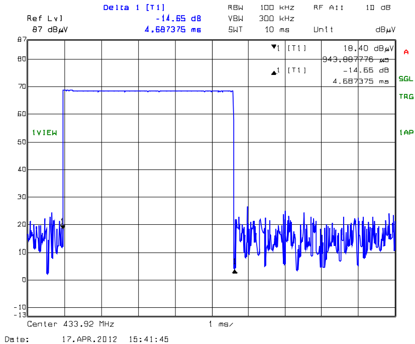
Plot 5.2.3.2. Duty Cycle (pulse length is 4.687375 ms)
