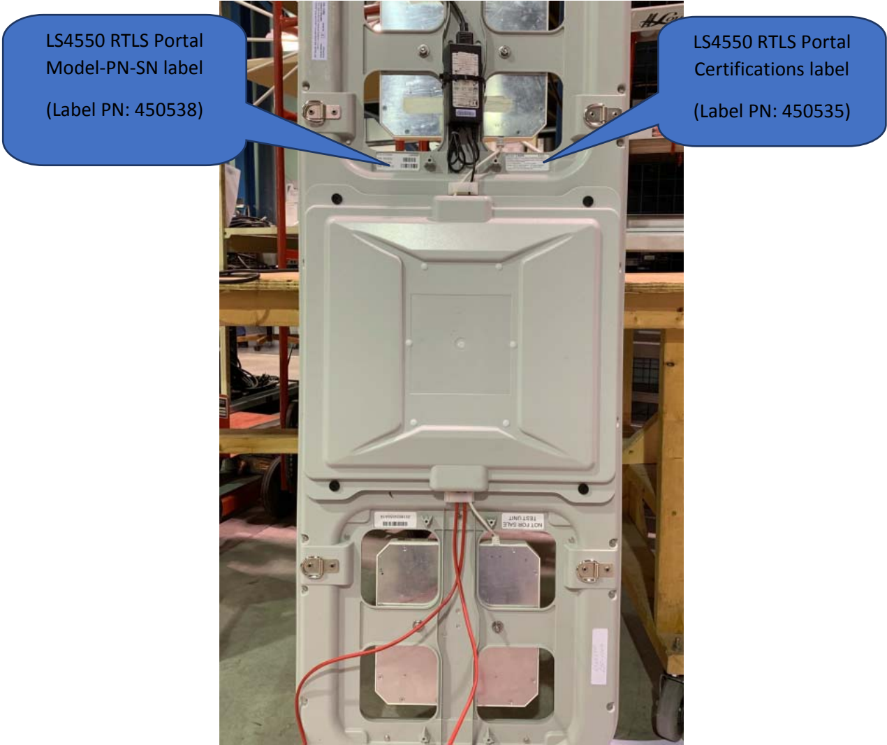
Figure 2 - LS4550 RTLS Portal back (top) view
