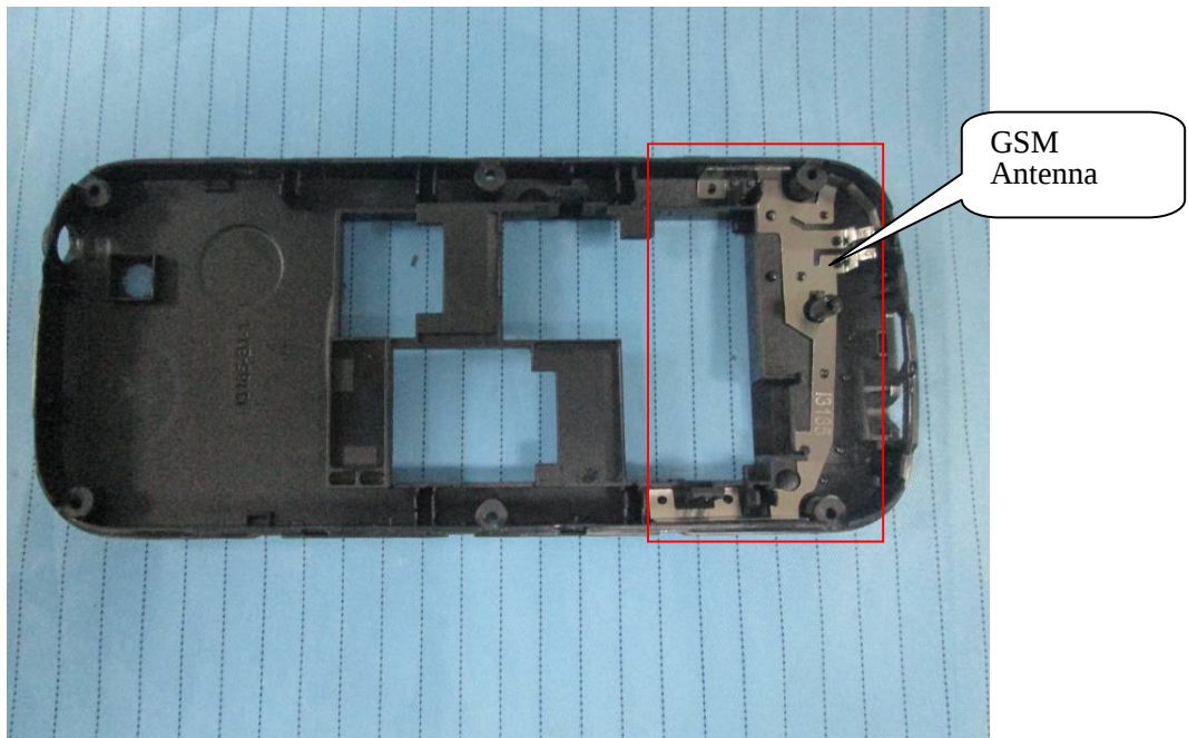
EUT –Antenna View 1
