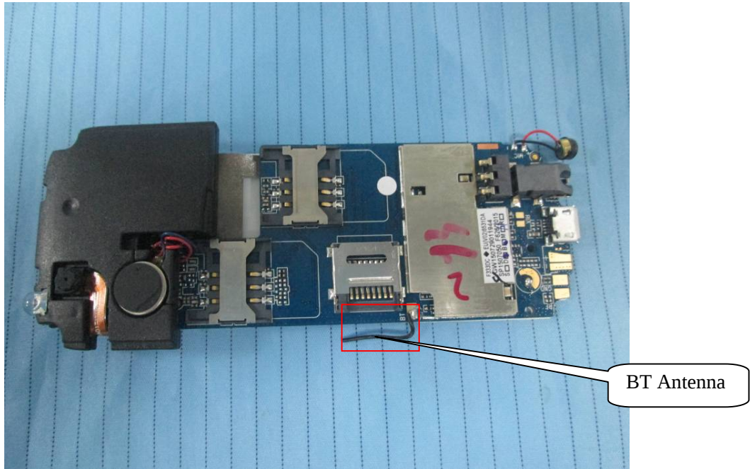
EUT –Antenna View 2
