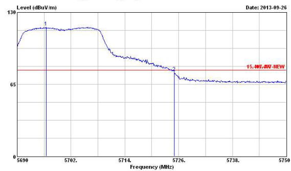
HT40-(Highest Ch.)
