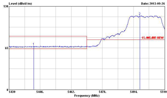
HT20-(Lowest Ch.)
