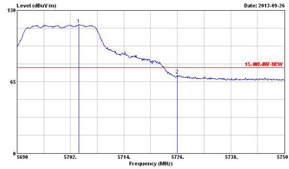
HT20-(Highest Ch.)
