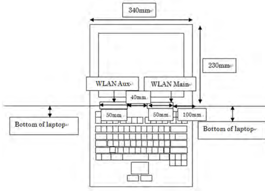
Fig.6 Antenna position of EUT (Back view)
