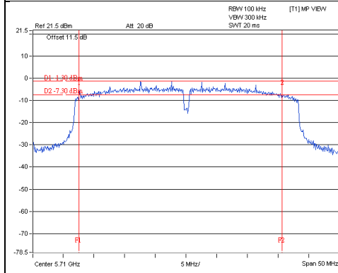
Chain 0 / CH142 (UNII-3 Band)
