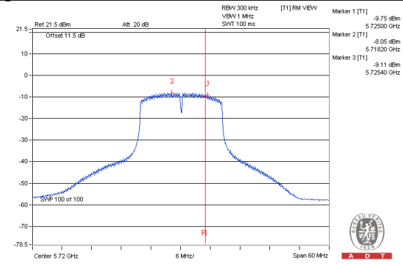
Chain 1 / CH144 (UNII-3 Band)
