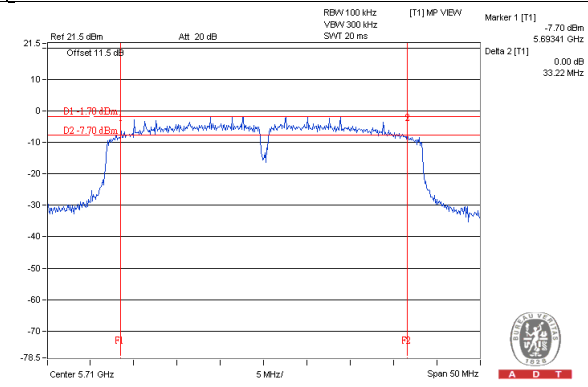
Chain 1 / CH142 (UNII-3 Band)
