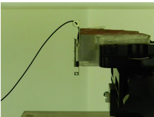
Right Side, Test Separation 0.9 cm
