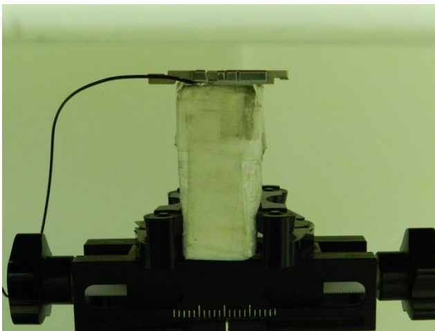
Bottom Side, Test Separation 0.9 cm
