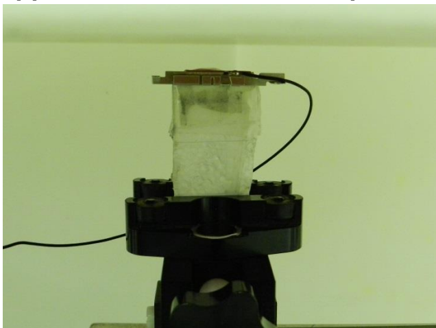
Top Side, Test Separation 0.9 cm
